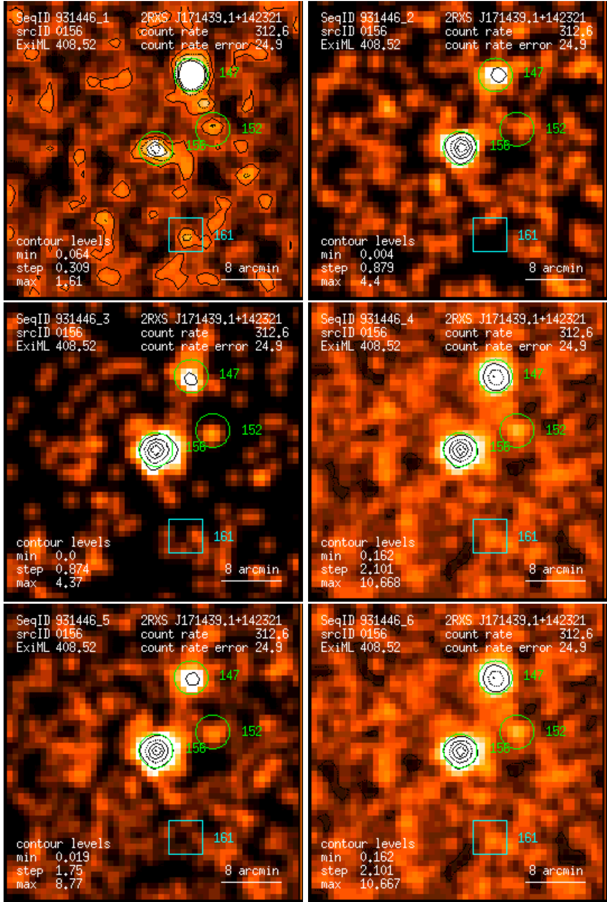
Figure 156: RASS 931446: detection 0156: band rate images, Gaussian filter: (1) PSPC channels 11 – 41, (2) 52 – 90, (3) 91 – 201, (4) 11 – 235, (5) 52 – 201, (6) 11 – 201. Broad band rates in counts/ks. Band rate contour levels in counts/ks/arcmin 2 .
