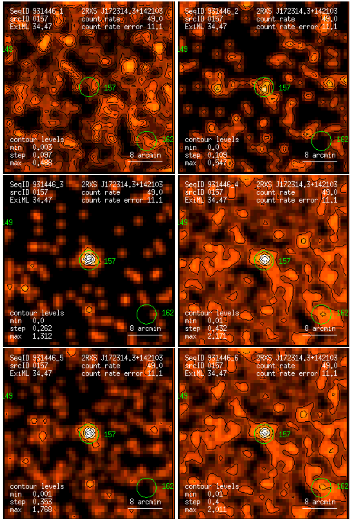
Figure 157: RASS 931446: detection 0157: band rate images, Gaussian filter: (1) PSPC channels 11 – 41, (2) 52 – 90, (3) 91 – 201, (4) 11 – 235, (5) 52 – 201, (6) 11 – 201. Broad band rates in counts/ks. Band rate contour levels in counts/ks/arcmin 2 .
