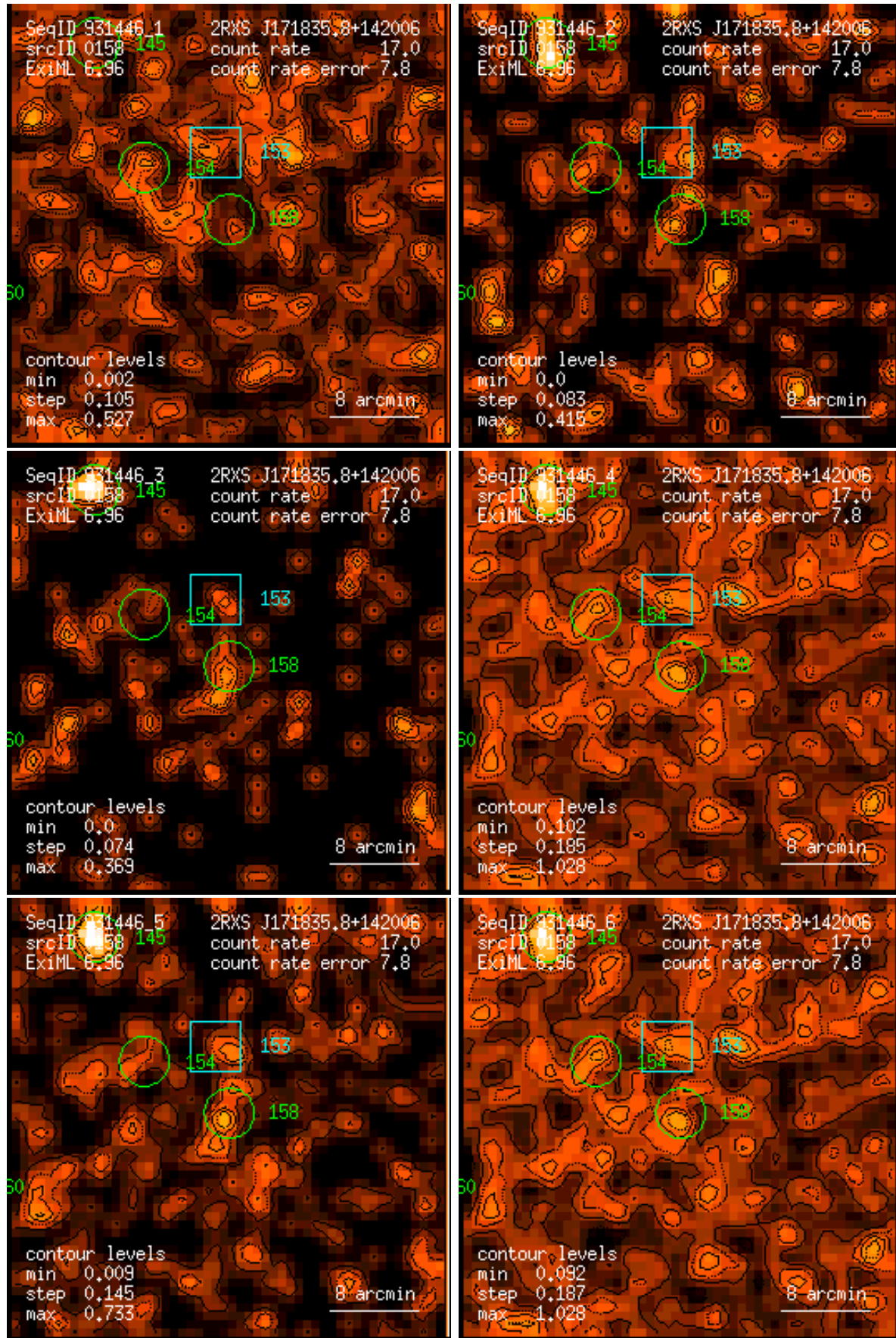
Figure 158: RASS 931446: detection 0158: band rate images, Gaussian filter: (1) PSPC channels 11 – 41, (2) 52 – 90, (3) 91 – 201, (4) 11 – 235, (5) 52 – 201, (6) 11 – 201. Broad band rates in counts/ks. Band rate contour levels in counts/ks/arcmin 2 .
