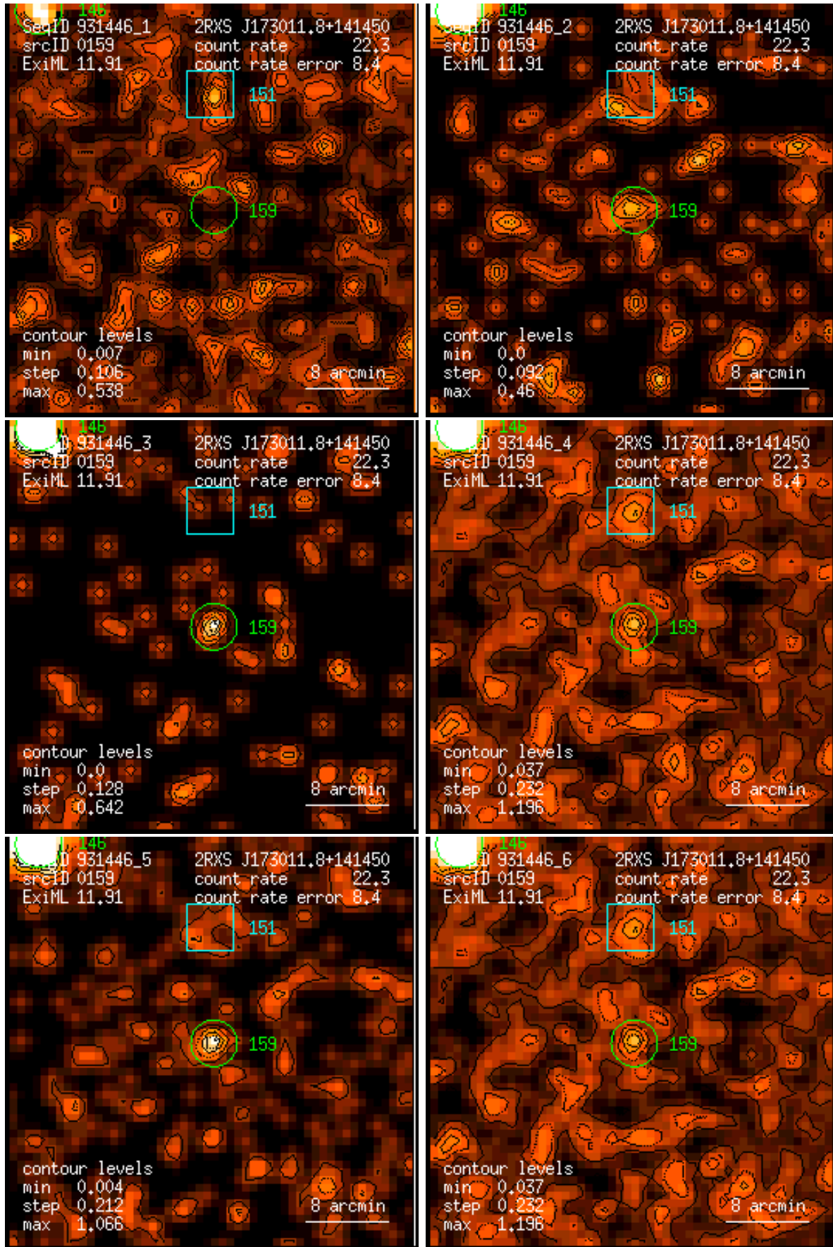
Figure 159: RASS 931446: detection 0159: band rate images, Gaussian filter: (1) PSPC channels 11 – 41, (2) 52 – 90, (3) 91 – 201, (4) 11 – 235, (5) 52 – 201, (6) 11 – 201. Broad band rates in counts/ks. Band rate contour levels in counts/ks/arcmin 2 .
