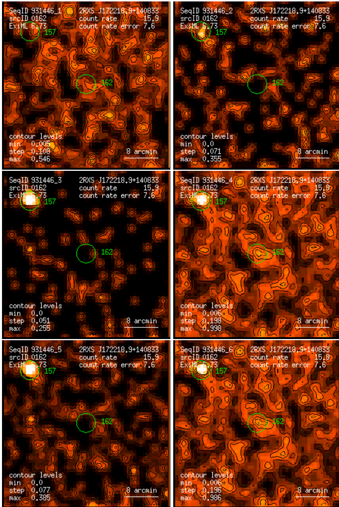
Figure 162: RASS 931446: detection 0162: band rate images, Gaussian filter: (1) PSPC channels 11 – 41, (2) 52 – 90, (3) 91 – 201, (4) 11 – 235, (5) 52 – 201, (6) 11 – 201. Broad band rates in counts/ks. Band rate contour levels in counts/ks/arcmin 2 .
