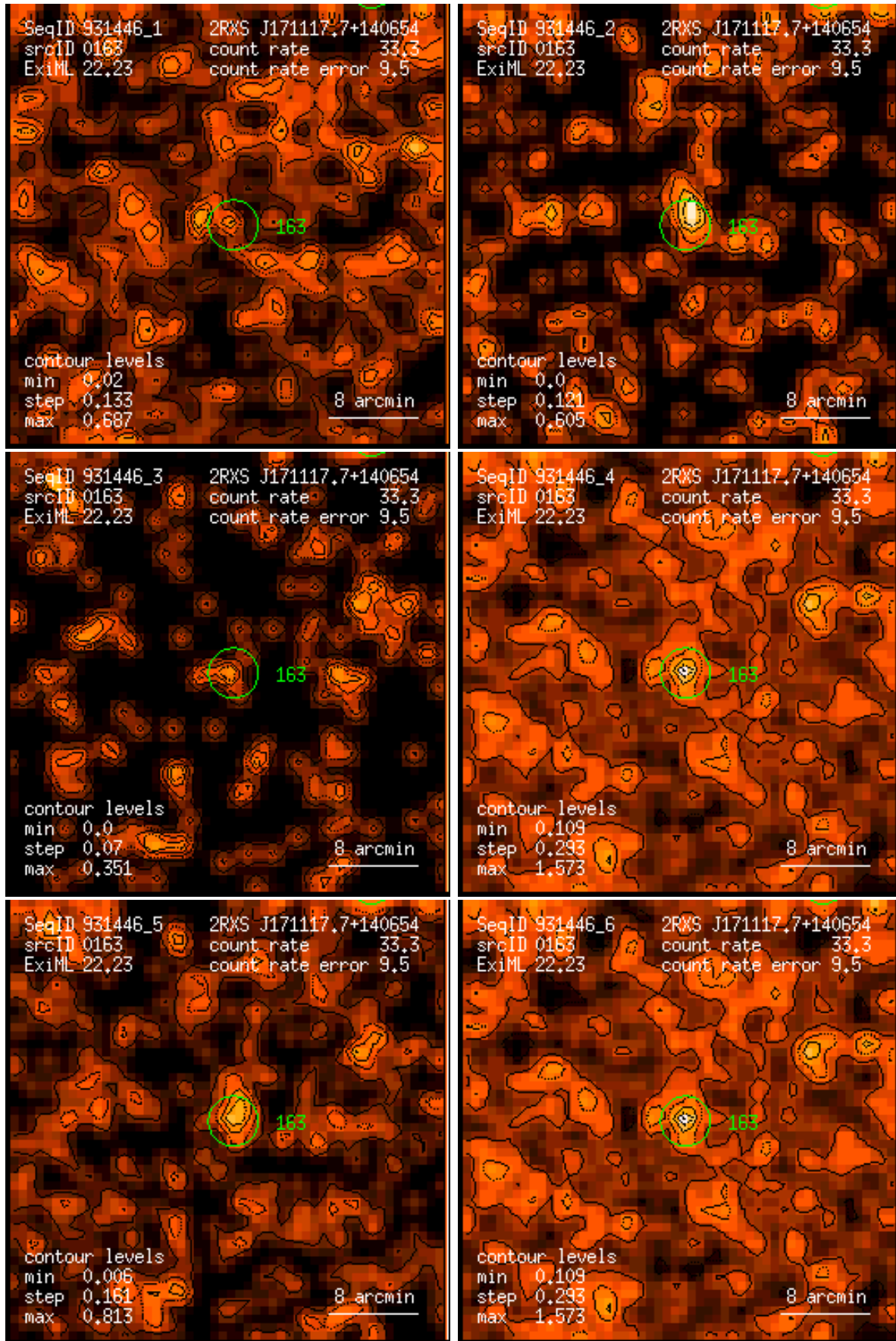
Figure 163: RASS 931446: detection 0163: band rate images, Gaussian filter: (1) PSPC channels 11 – 41, (2) 52 – 90, (3) 91 – 201, (4) 11 – 235, (5) 52 – 201, (6) 11 – 201. Broad band rates in counts/ks. Band rate contour levels in counts/ks/arcmin 2 .
