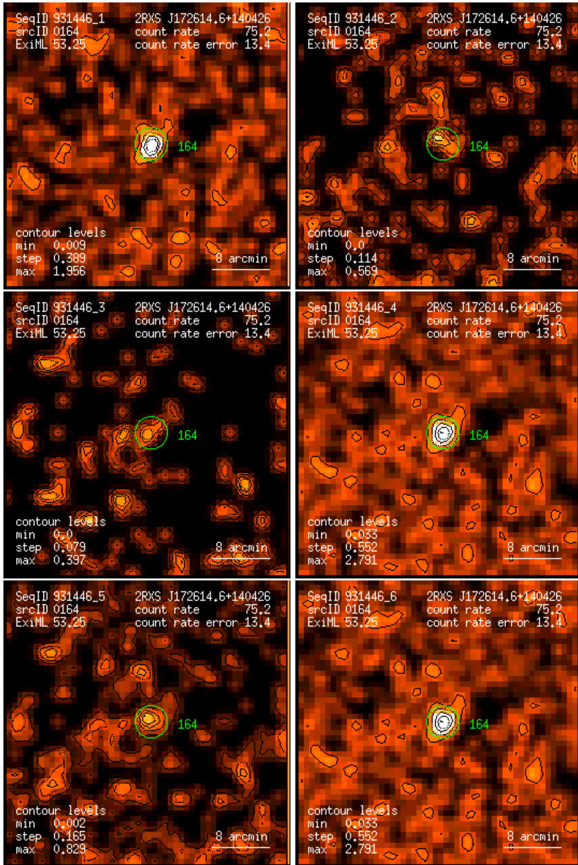
Figure 164: RASS 931446: detection 0164: band rate images, Gaussian filter: (1) PSPC channels 11 – 41, (2) 52 – 90, (3) 91 – 201, (4) 11 – 235, (5) 52 – 201, (6) 11 – 201. Broad band rates in counts/ks. Band rate contour levels in counts/ks/arcmin 2 .
