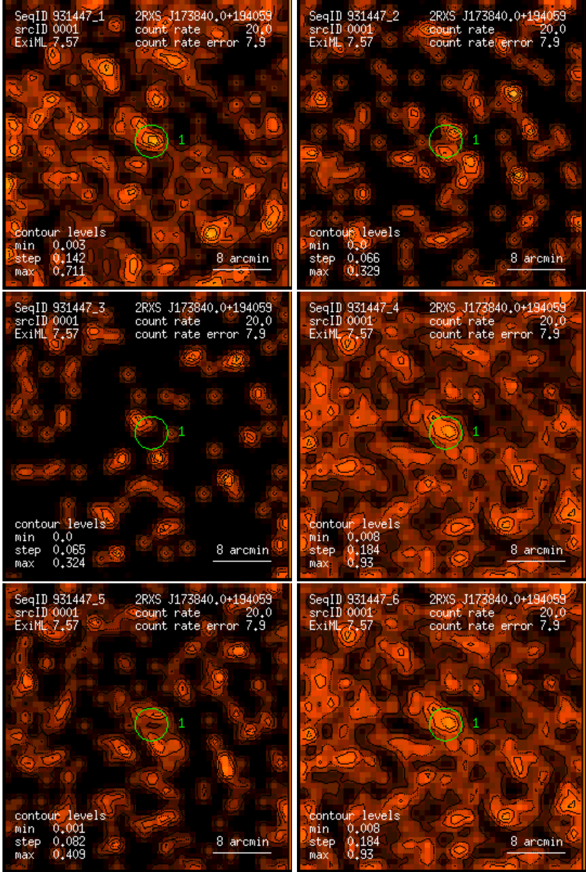
Figure 1: RASS 931447: detection 0001: band rate images, Gaussian filter: (1) PSPC channels 11 – 41, (2) 52 – 90, (3) 91 – 201, (4) 11 – 235, (5) 52 – 201, (6) 11 – 201. Broad band rates in counts/ks. Band rate contour levels in counts/ks/arcmin 2 .
