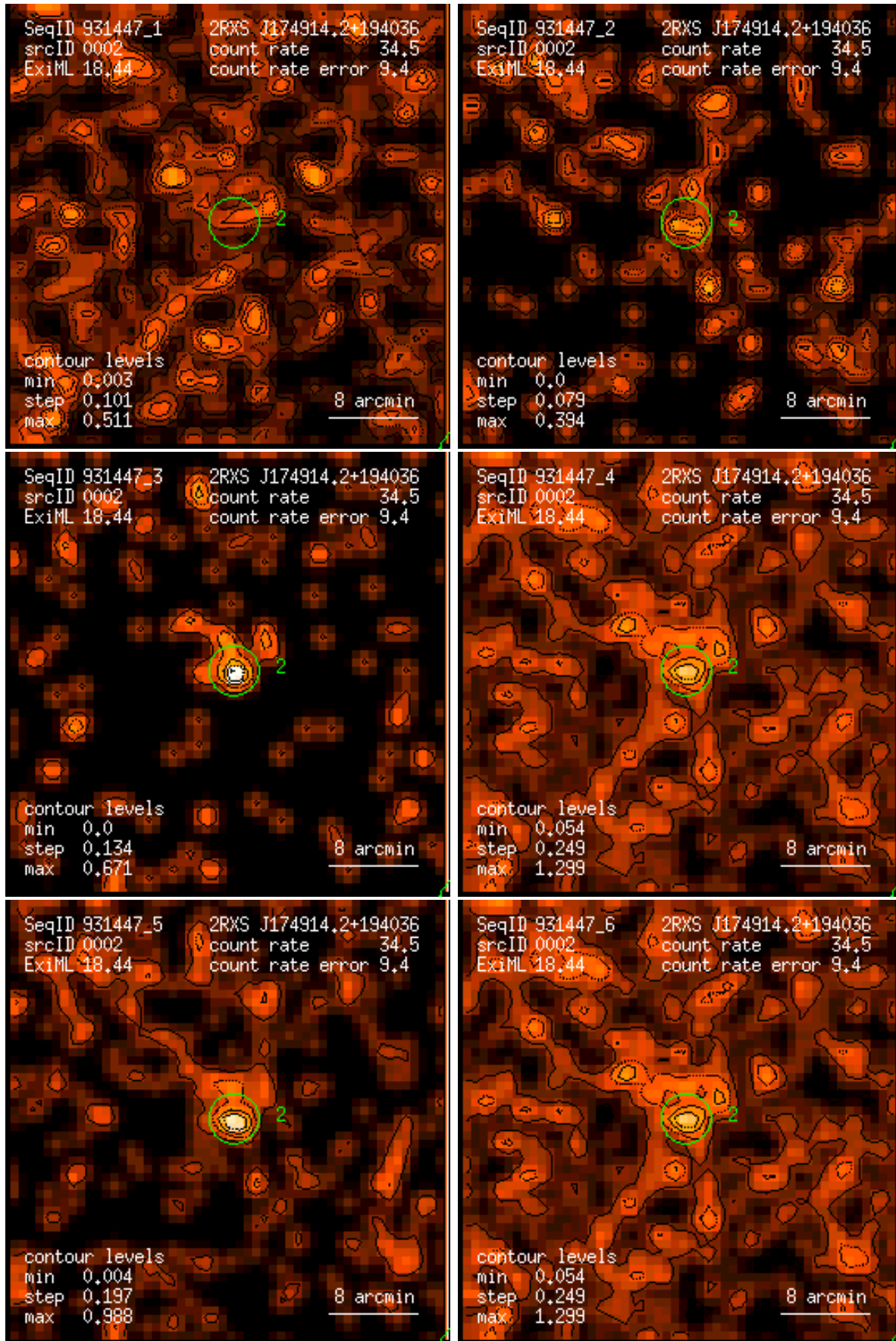
Figure 2: RASS 931447: detection 0002: band rate images, Gaussian filter: (1) PSPC channels 11 – 41, (2) 52 – 90, (3) 91 – 201, (4) 11 – 235, (5) 52 – 201, (6) 11 – 201. Broad band rates in counts/ks. Band rate contour levels in counts/ks/arcmin 2 .
