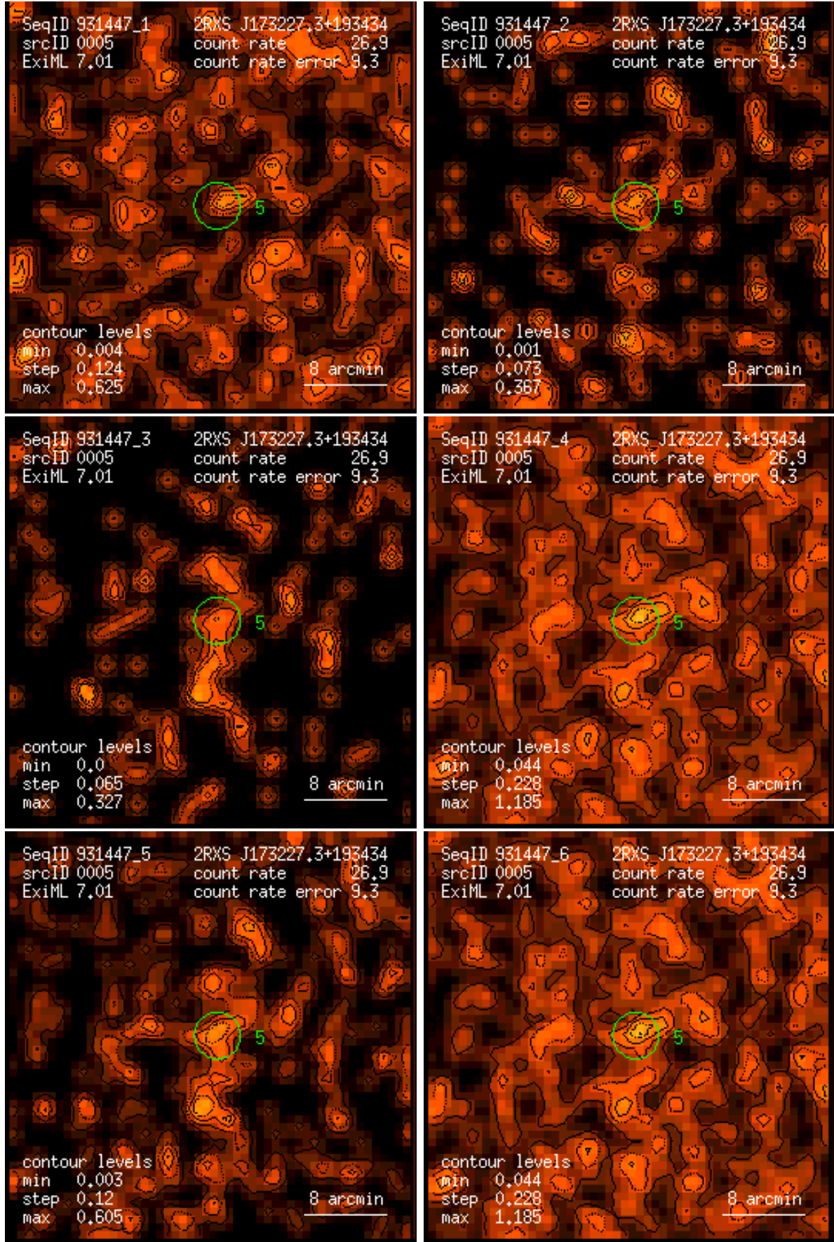
Figure 5: RASS 931447: detection 0005: band rate images, Gaussian filter: (1) PSPC channels 11 – 41, (2) 52 – 90, (3) 91 – 201, (4) 11 – 235, (5) 52 – 201, (6) 11 – 201. Broad band rates in counts/ks. Band rate contour levels in counts/ks/arcmin 2 .
