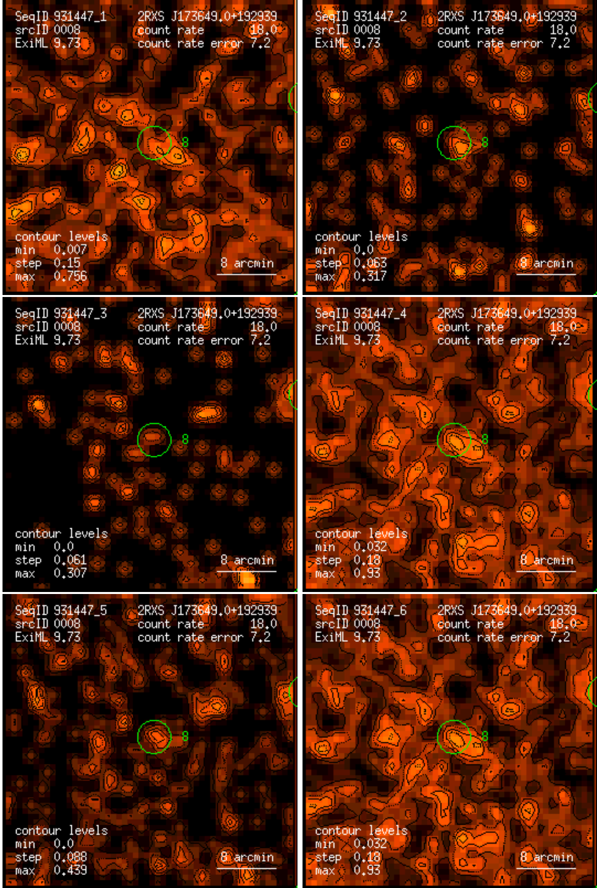
Figure 8: RASS 931447: detection 0008: band rate images, Gaussian filter: (1) PSPC channels 11 – 41, (2) 52 – 90, (3) 91 – 201, (4) 11 – 235, (5) 52 – 201, (6) 11 – 201. Broad band rates in counts/ks. Band rate contour levels in counts/ks/arcmin 2 .
