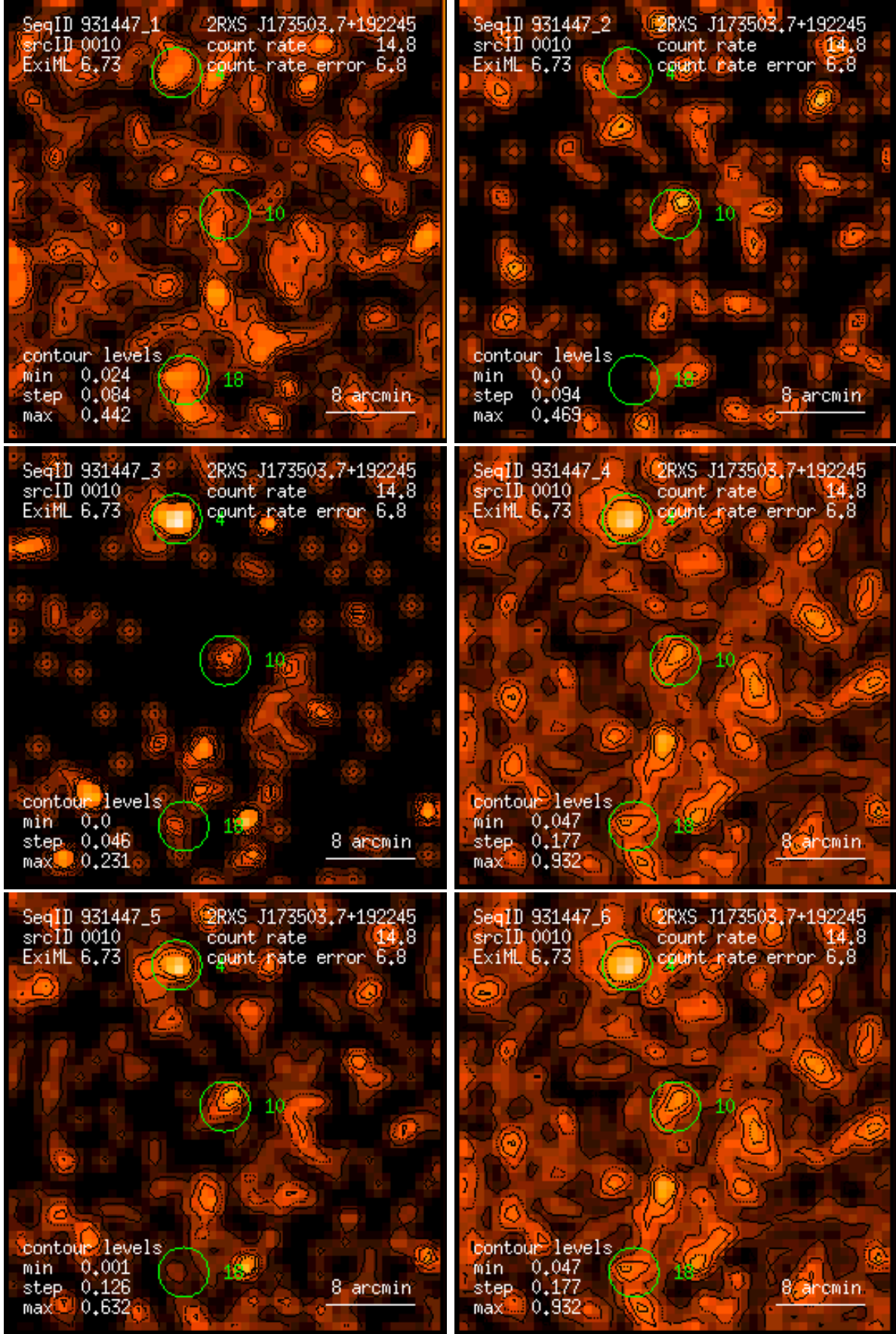
Figure 10: RASS 931447: detection 0010: band rate images, Gaussian filter: (1) PSPC channels 11 – 41, (2) 52 – 90, (3) 91 – 201, (4) 11 – 235, (5) 52 – 201, (6) 11 – 201. Broad band rates in counts/ks. Band rate contour levels in counts/ks/arcmin 2 .
