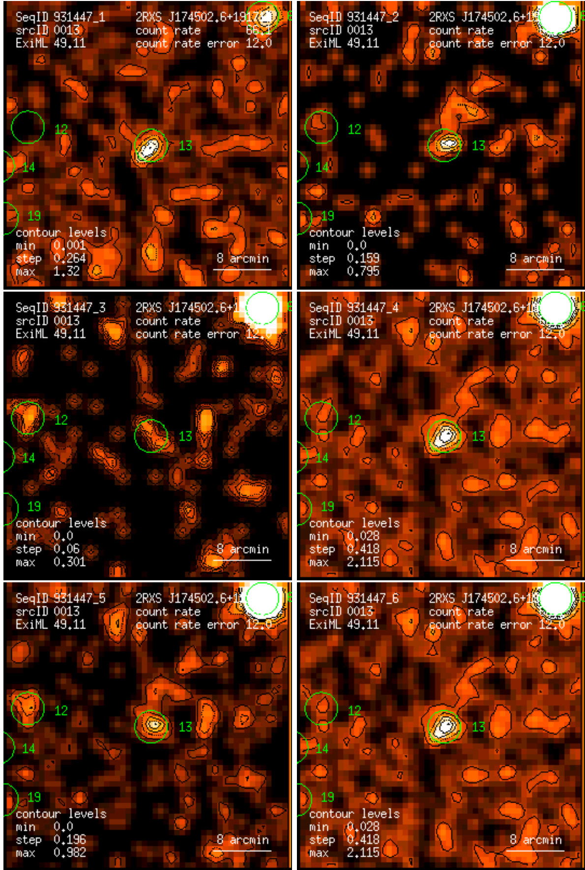
Figure 13: RASS 931447: detection 0013: band rate images, Gaussian filter: (1) PSPC channels 11 – 41, (2) 52 – 90, (3) 91 – 201, (4) 11 – 235, (5) 52 – 201, (6) 11 – 201. Broad band rates in counts/ks. Band rate contour levels in counts/ks/arcmin 2 .
