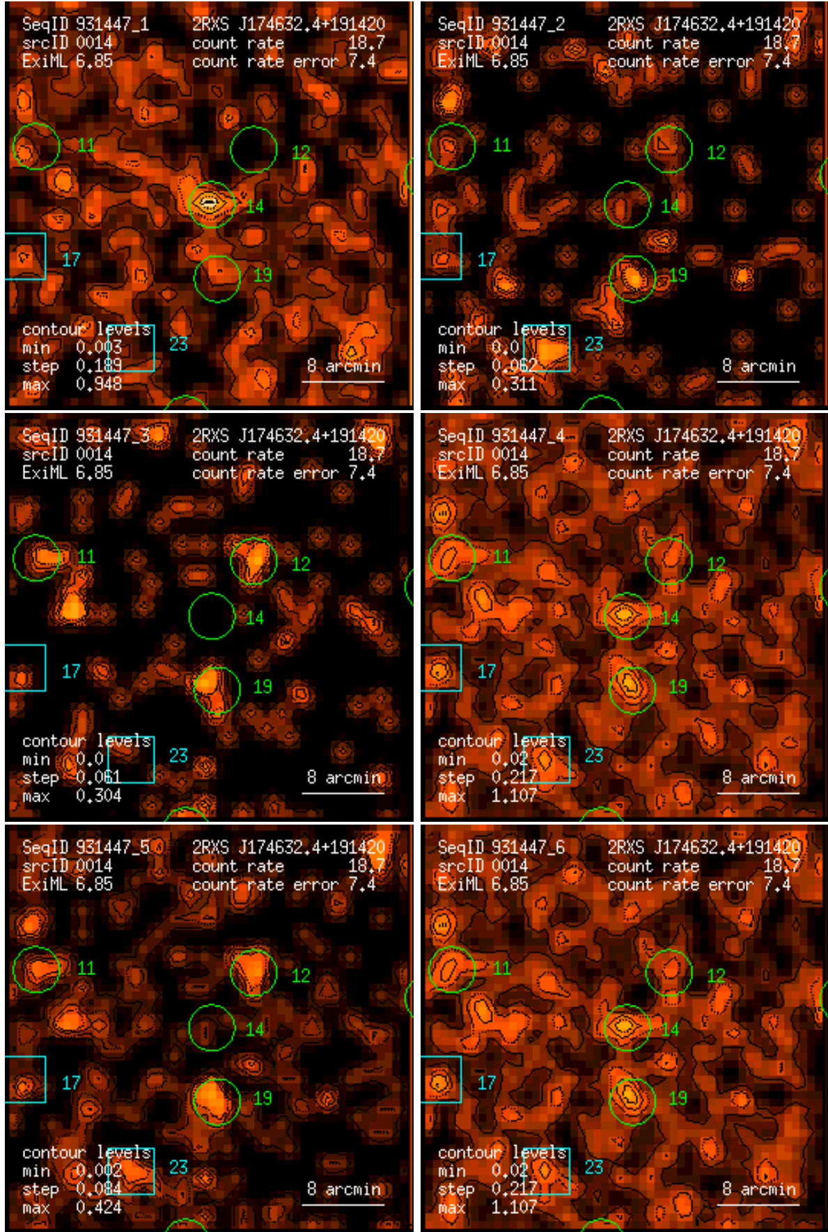
Figure 14: RASS 931447: detection 0014: band rate images, Gaussian filter: (1) PSPC channels 11 – 41, (2) 52 – 90, (3) 91 – 201, (4) 11 – 235, (5) 52 – 201, (6) 11 – 201. Broad band rates in counts/ks. Band rate contour levels in counts/ks/arcmin 2 .
