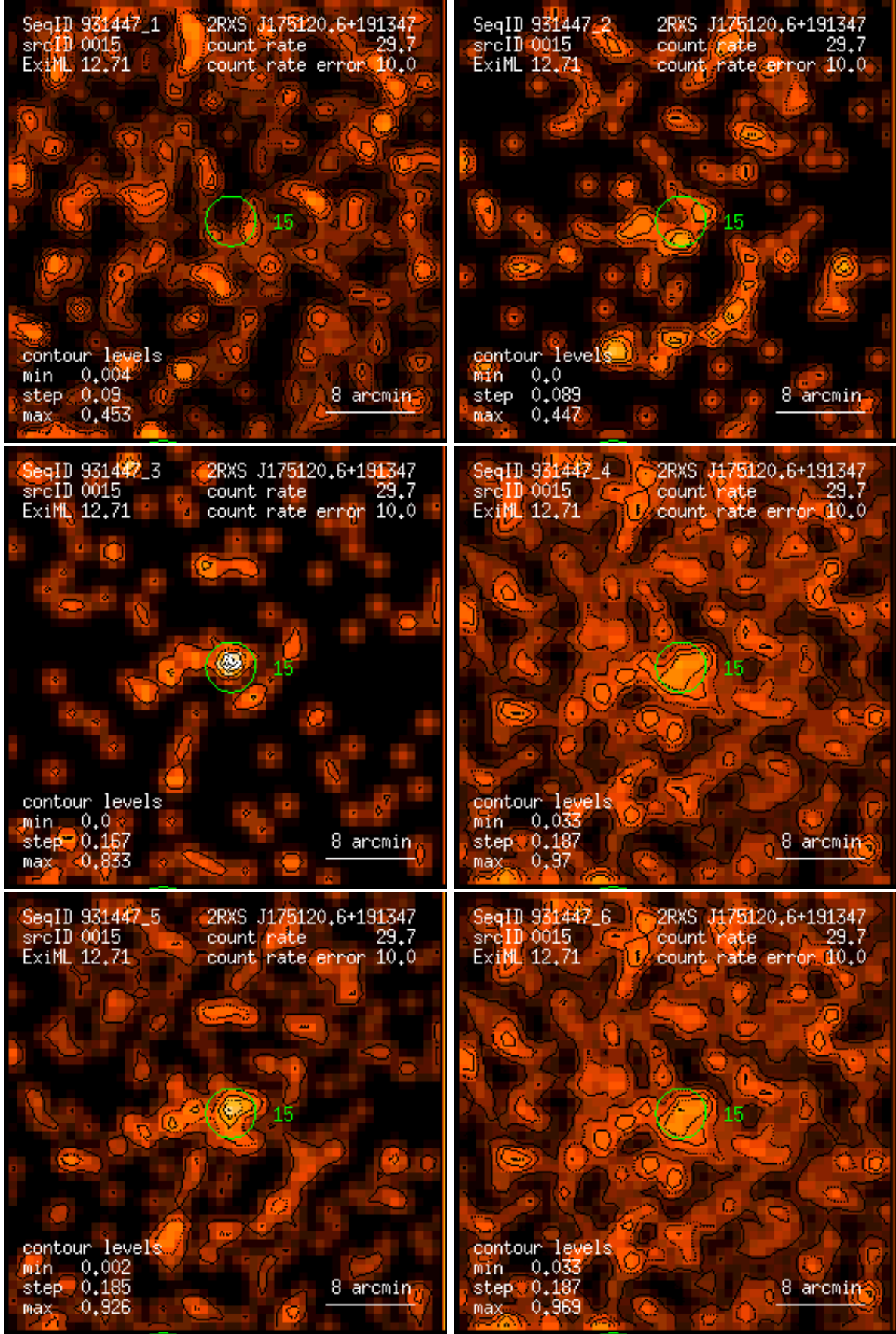
Figure 15: RASS 931447: detection 0015: band rate images, Gaussian filter: (1) PSPC channels 11 – 41, (2) 52 – 90, (3) 91 – 201, (4) 11 – 235, (5) 52 – 201, (6) 11 – 201. Broad band rates in counts/ks. Band rate contour levels in counts/ks/arcmin 2 .
