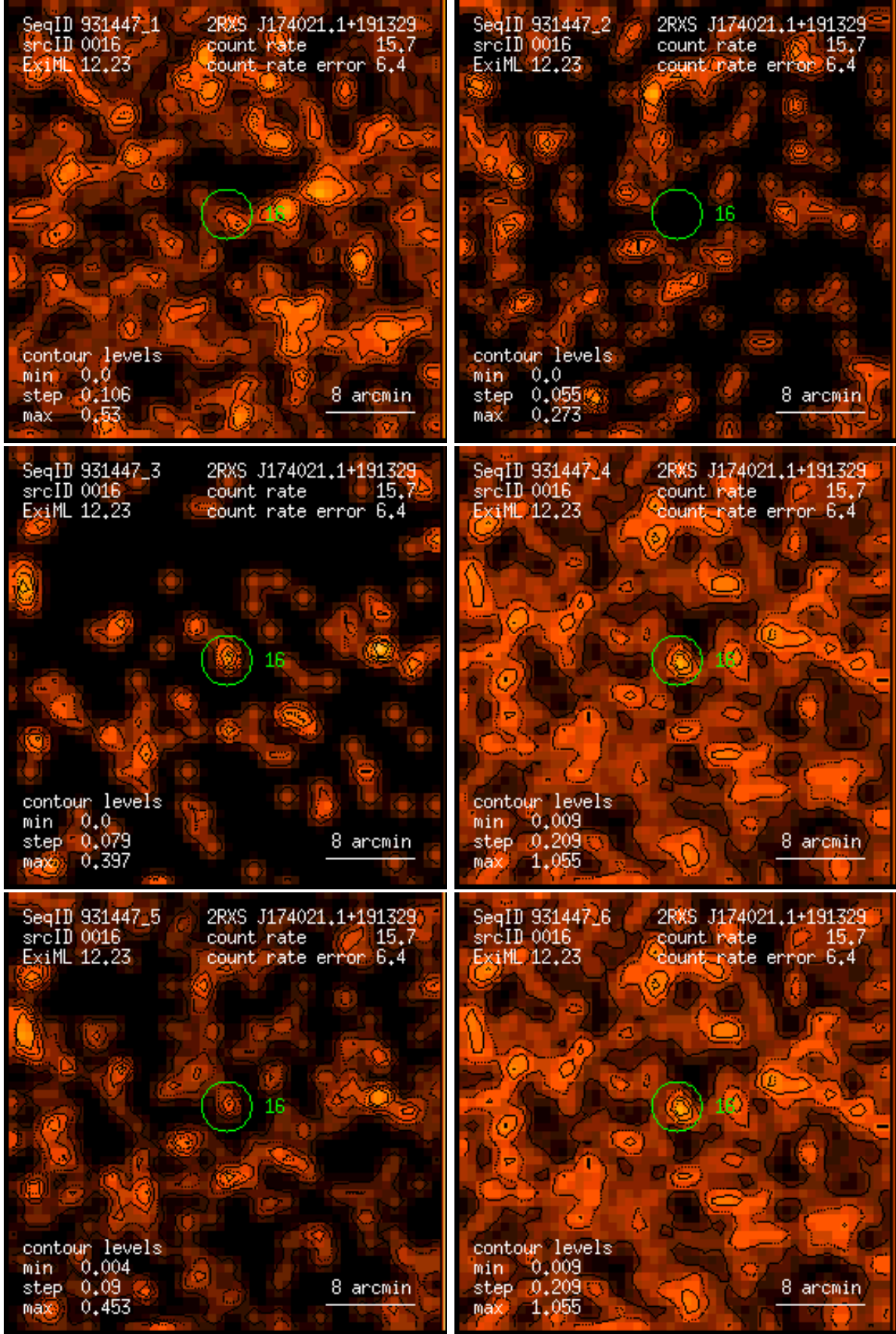
Figure 16: RASS 931447: detection 0016: band rate images, Gaussian filter: (1) PSPC channels 11 – 41, (2) 52 – 90, (3) 91 – 201, (4) 11 – 235, (5) 52 – 201, (6) 11 – 201. Broad band rates in counts/ks. Band rate contour levels in counts/ks/arcmin 2 .
