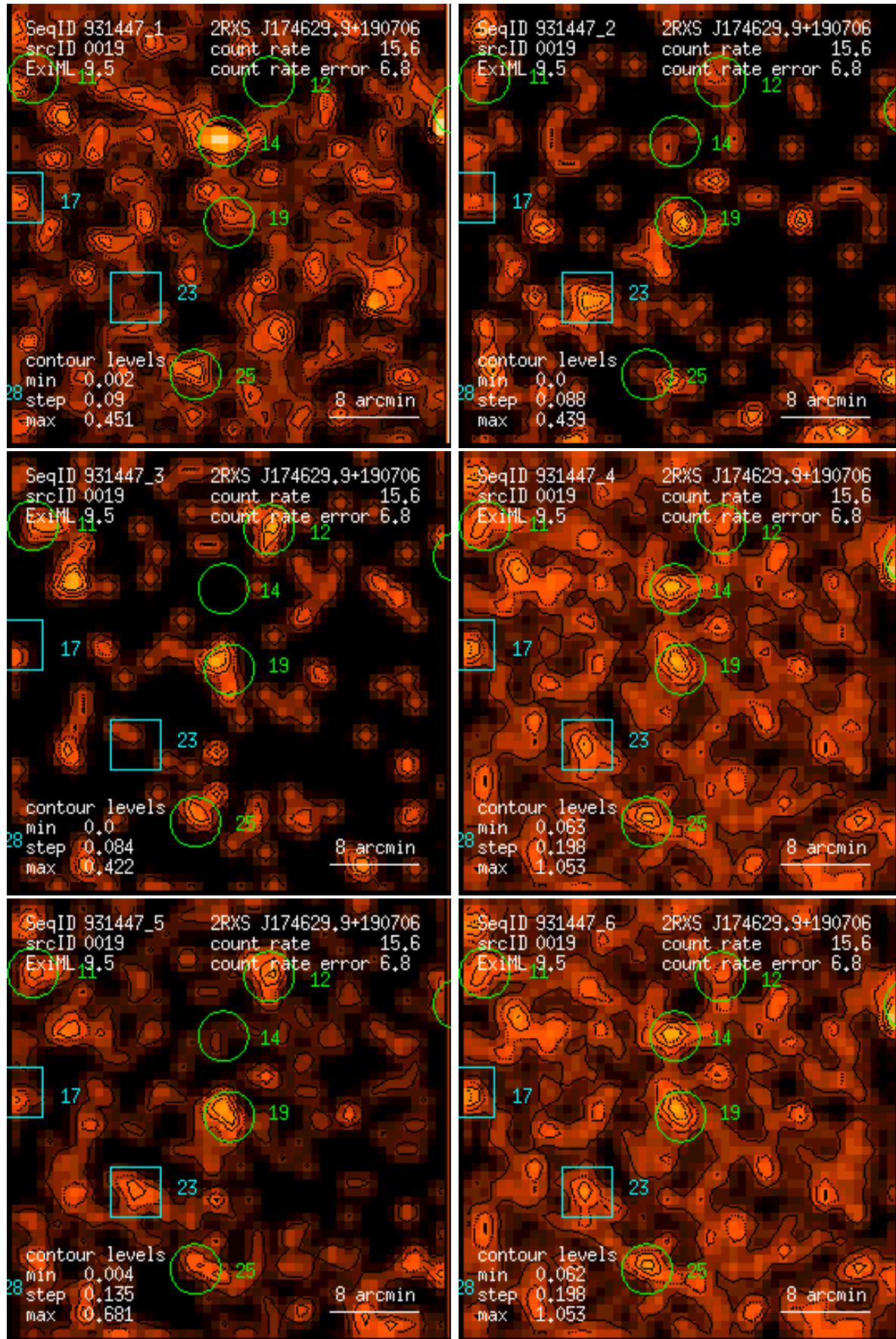
Figure 19: RASS 931447: detection 0019: band rate images, Gaussian filter: (1) PSPC channels 11 – 41, (2) 52 – 90, (3) 91 – 201, (4) 11 – 235, (5) 52 – 201, (6) 11 – 201. Broad band rates in counts/ks. Band rate contour levels in counts/ks/arcmin 2 .
