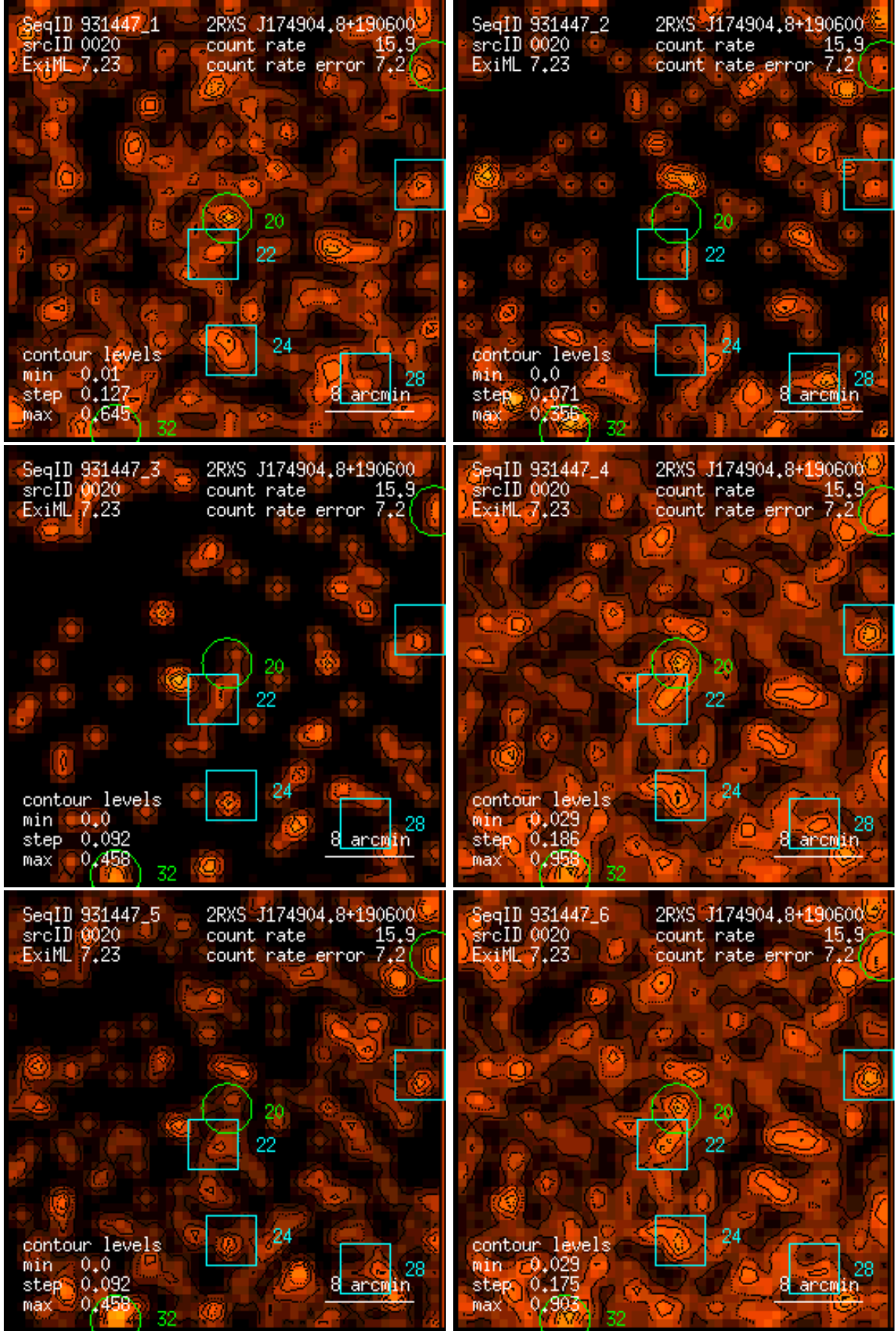
Figure 20: RASS 931447: detection 0020: band rate images, Gaussian filter: (1) PSPC channels 11 – 41, (2) 52 – 90, (3) 91 – 201, (4) 11 – 235, (5) 52 – 201, (6) 11 – 201. Broad band rates in counts/ks. Band rate contour levels in counts/ks/arcmin 2 .
