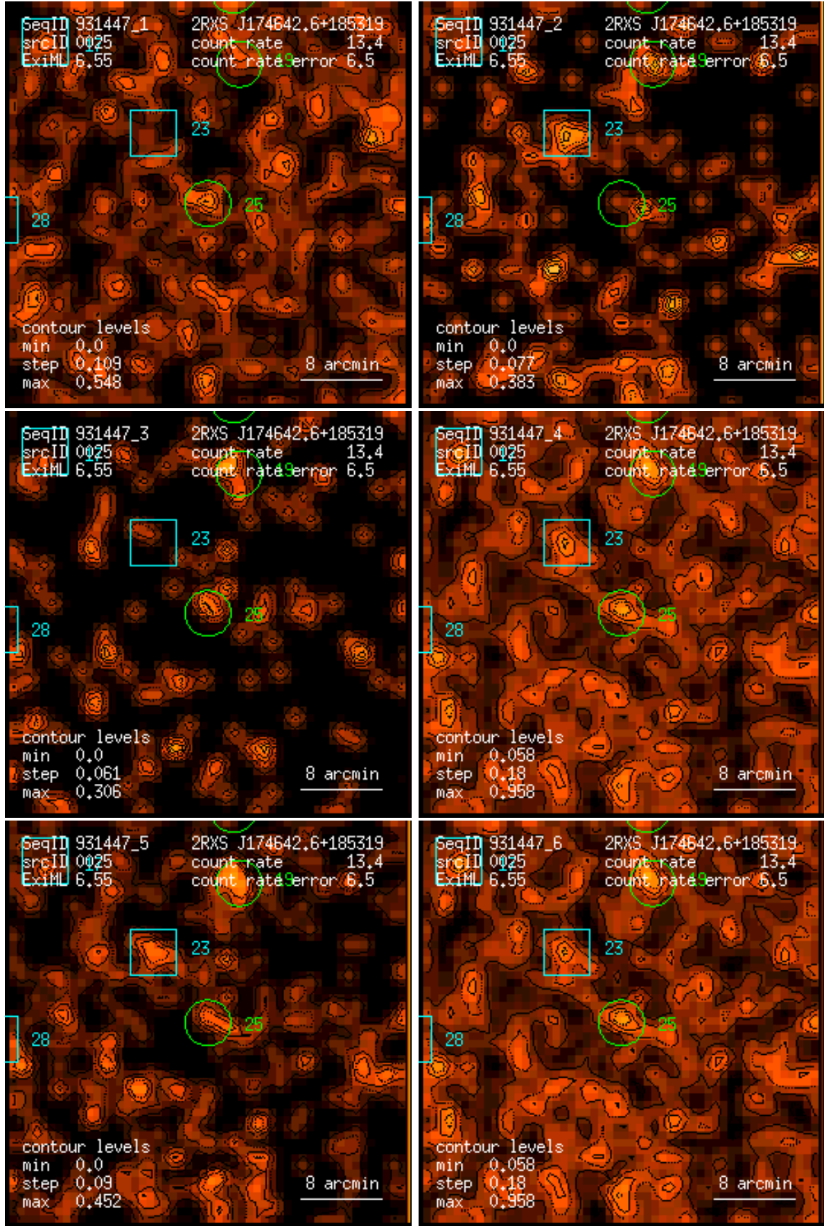
Figure 25: RASS 931447: detection 0025: band rate images, Gaussian filter: (1) PSPC channels 11 – 41, (2) 52 – 90, (3) 91 – 201, (4) 11 – 235, (5) 52 – 201, (6) 11 – 201. Broad band rates in counts/ks. Band rate contour levels in counts/ks/arcmin 2 .
