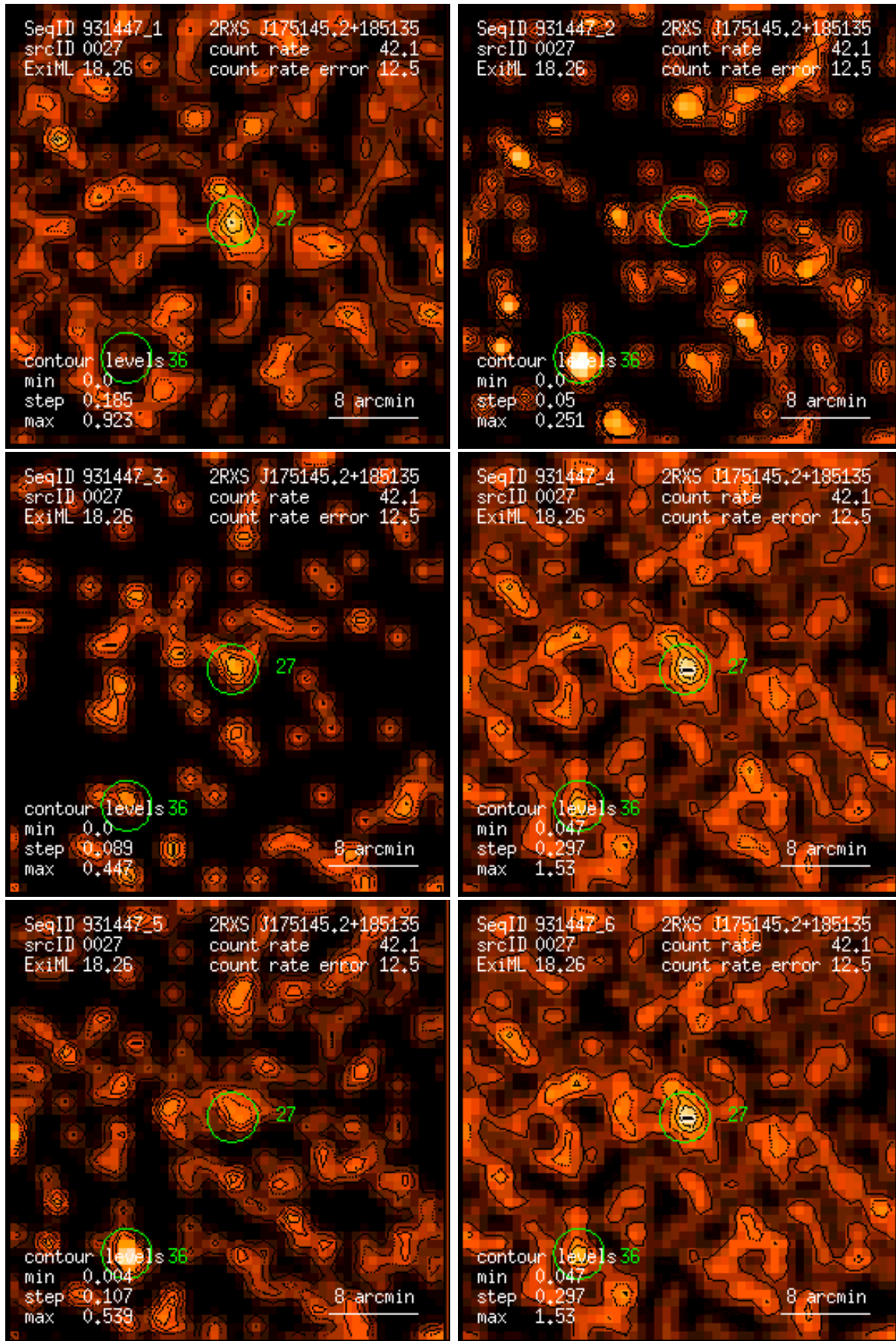
Figure 27: RASS 931447: detection 0027: band rate images, Gaussian filter: (1) PSPC channels 11 – 41, (2) 52 – 90, (3) 91 – 201, (4) 11 – 235, (5) 52 – 201, (6) 11 – 201. Broad band rates in counts/ks. Band rate contour levels in counts/ks/arcmin 2 .
