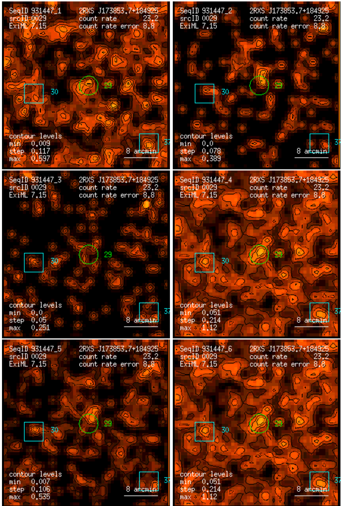
Figure 29: RASS 931447: detection 0029: band rate images, Gaussian filter: (1) PSPC channels 11 – 41, (2) 52 – 90, (3) 91 – 201, (4) 11 – 235, (5) 52 – 201, (6) 11 – 201. Broad band rates in counts/ks. Band rate contour levels in counts/ks/arcmin 2 .
