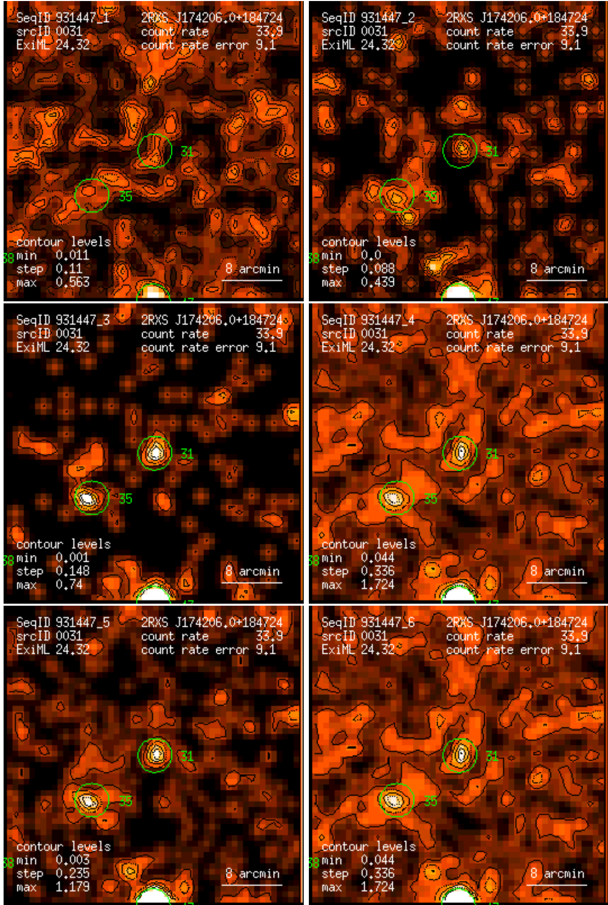
Figure 31: RASS 931447: detection 0031: band rate images, Gaussian filter: (1) PSPC channels 11 – 41, (2) 52 – 90, (3) 91 – 201, (4) 11 – 235, (5) 52 – 201, (6) 11 – 201. Broad band rates in counts/ks. Band rate contour levels in counts/ks/arcmin 2 .
