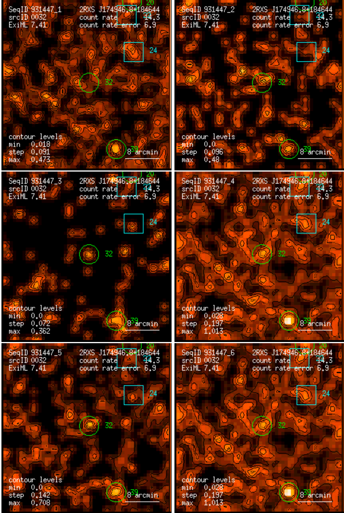
Figure 32: RASS 931447: detection 0032: band rate images, Gaussian filter: (1) PSPC channels 11 – 41, (2) 52 – 90, (3) 91 – 201, (4) 11 – 235, (5) 52 – 201, (6) 11 – 201. Broad band rates in counts/ks. Band rate contour levels in counts/ks/arcmin 2 .
