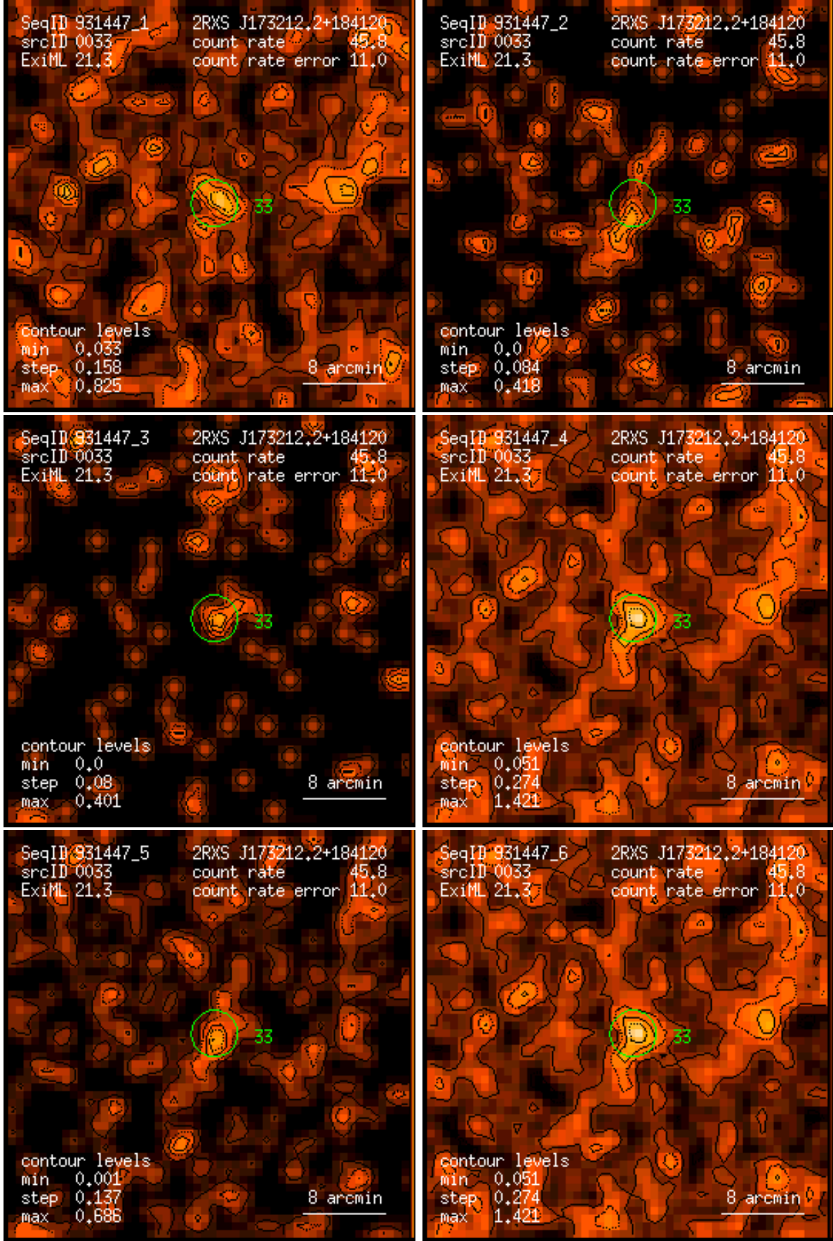
Figure 33: RASS 931447: detection 0033: band rate images, Gaussian filter: (1) PSPC channels 11 – 41, (2) 52 – 90, (3) 91 – 201, (4) 11 – 235, (5) 52 – 201, (6) 11 – 201. Broad band rates in counts/ks. Band rate contour levels in counts/ks/arcmin 2 .
