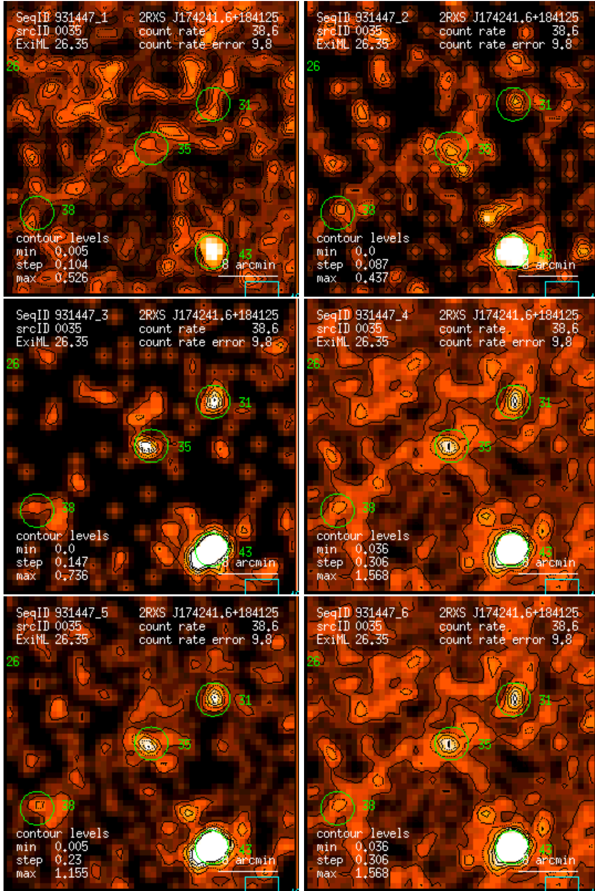
Figure 35: RASS 931447: detection 0035: band rate images, Gaussian filter: (1) PSPC channels 11 – 41, (2) 52 – 90, (3) 91 – 201, (4) 11 – 235, (5) 52 – 201, (6) 11 – 201. Broad band rates in counts/ks. Band rate contour levels in counts/ks/arcmin 2 .
