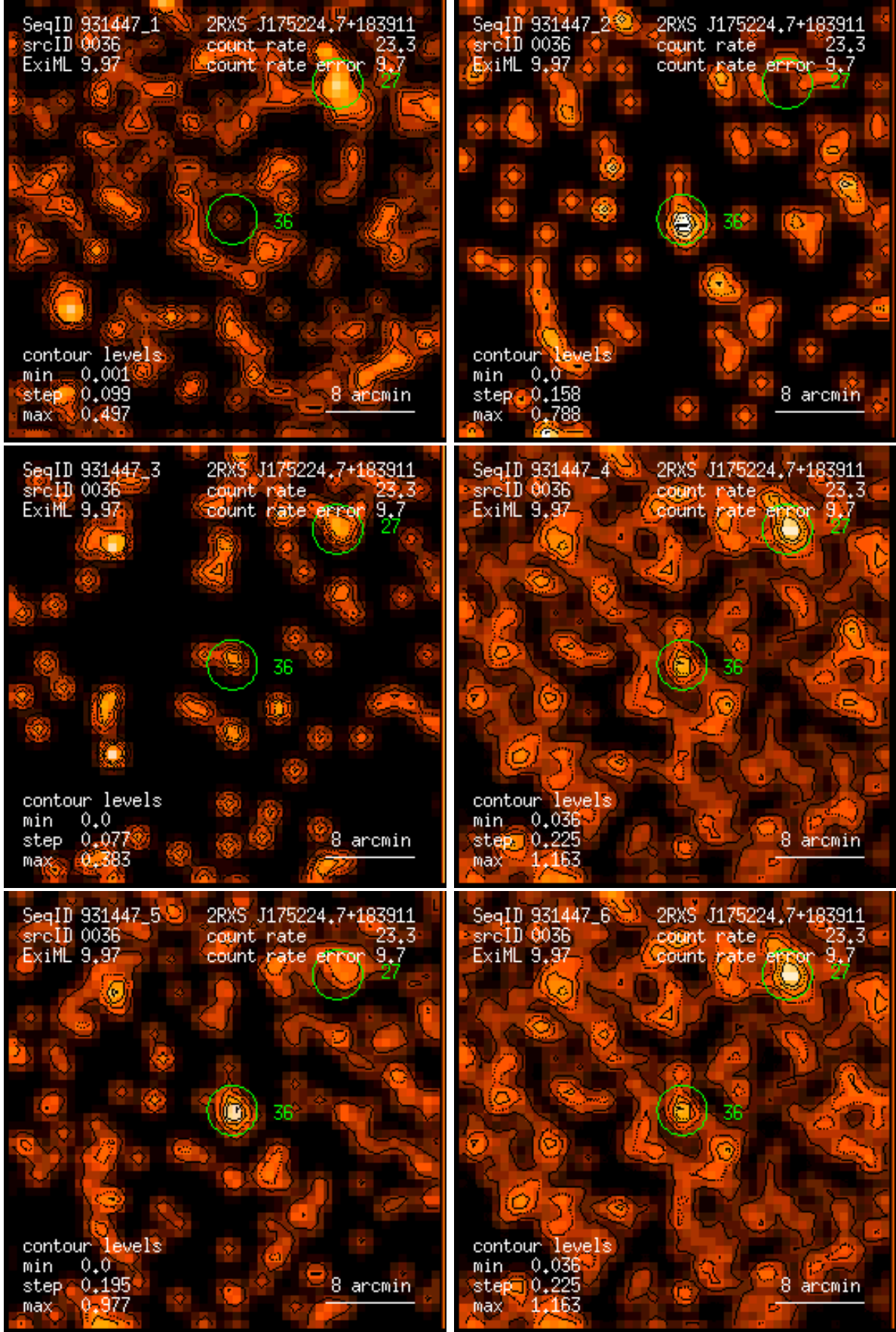
Figure 36: RASS 931447: detection 0036: band rate images, Gaussian filter: (1) PSPC channels 11 – 41, (2) 52 – 90, (3) 91 – 201, (4) 11 – 235, (5) 52 – 201, (6) 11 – 201. Broad band rates in counts/ks. Band rate contour levels in counts/ks/arcmin 2 .
