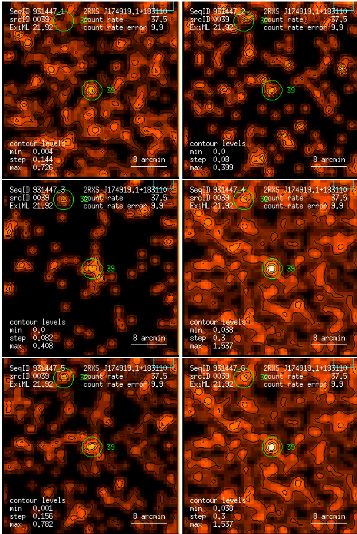
Figure 39: RASS 931447: detection 0039: band rate images, Gaussian filter: (1) PSPC channels 11 – 41, (2) 52 – 90, (3) 91 – 201, (4) 11 – 235, (5) 52 – 201, (6) 11 – 201. Broad band rates in counts/ks. Band rate contour levels in counts/ks/arcmin 2 .
