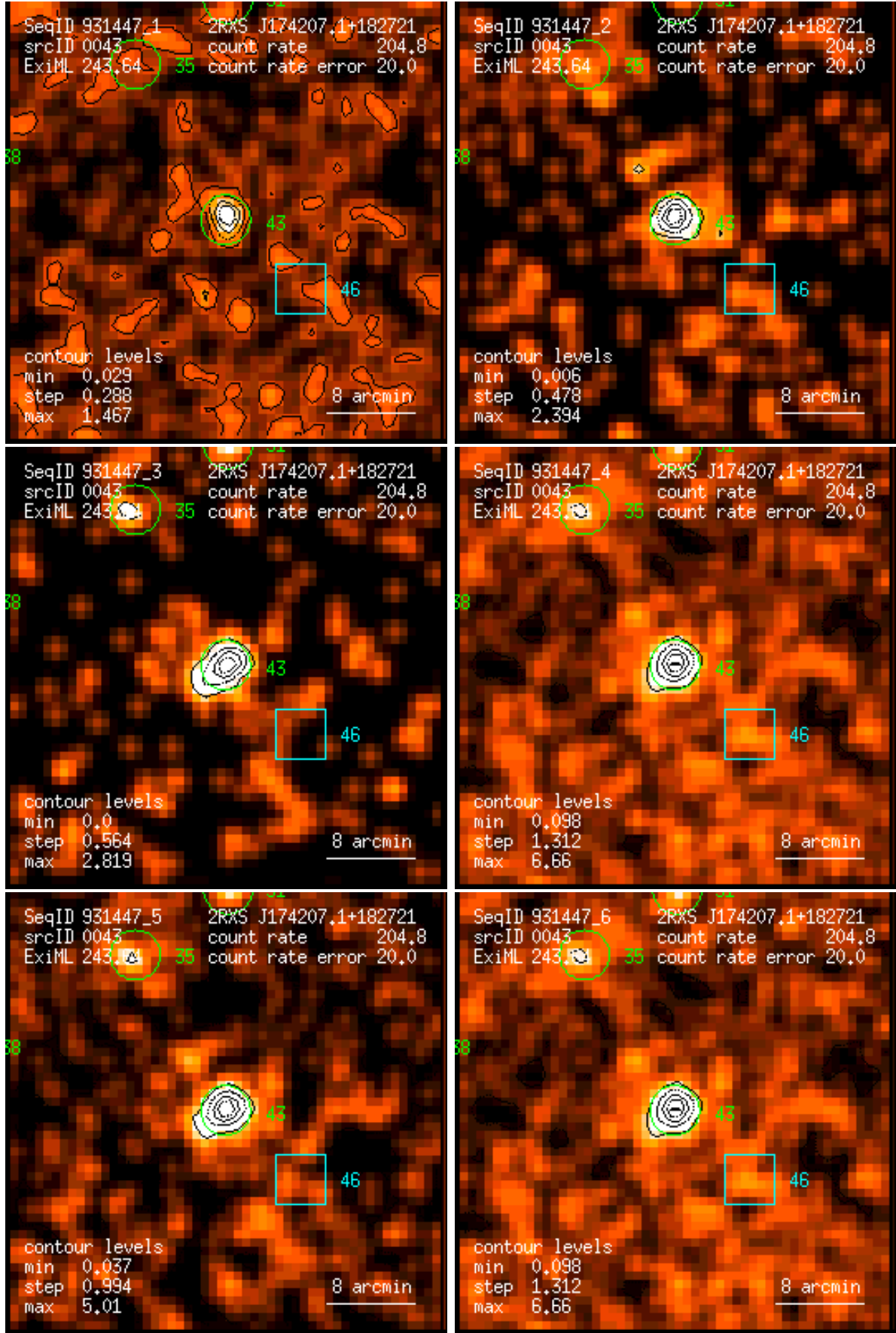
Figure 43: RASS 931447: detection 0043: band rate images, Gaussian filter: (1) PSPC channels 11 – 41, (2) 52 – 90, (3) 91 – 201, (4) 11 – 235, (5) 52 – 201, (6) 11 – 201. Broad band rates in counts/ks. Band rate contour levels in counts/ks/arcmin 2 .
