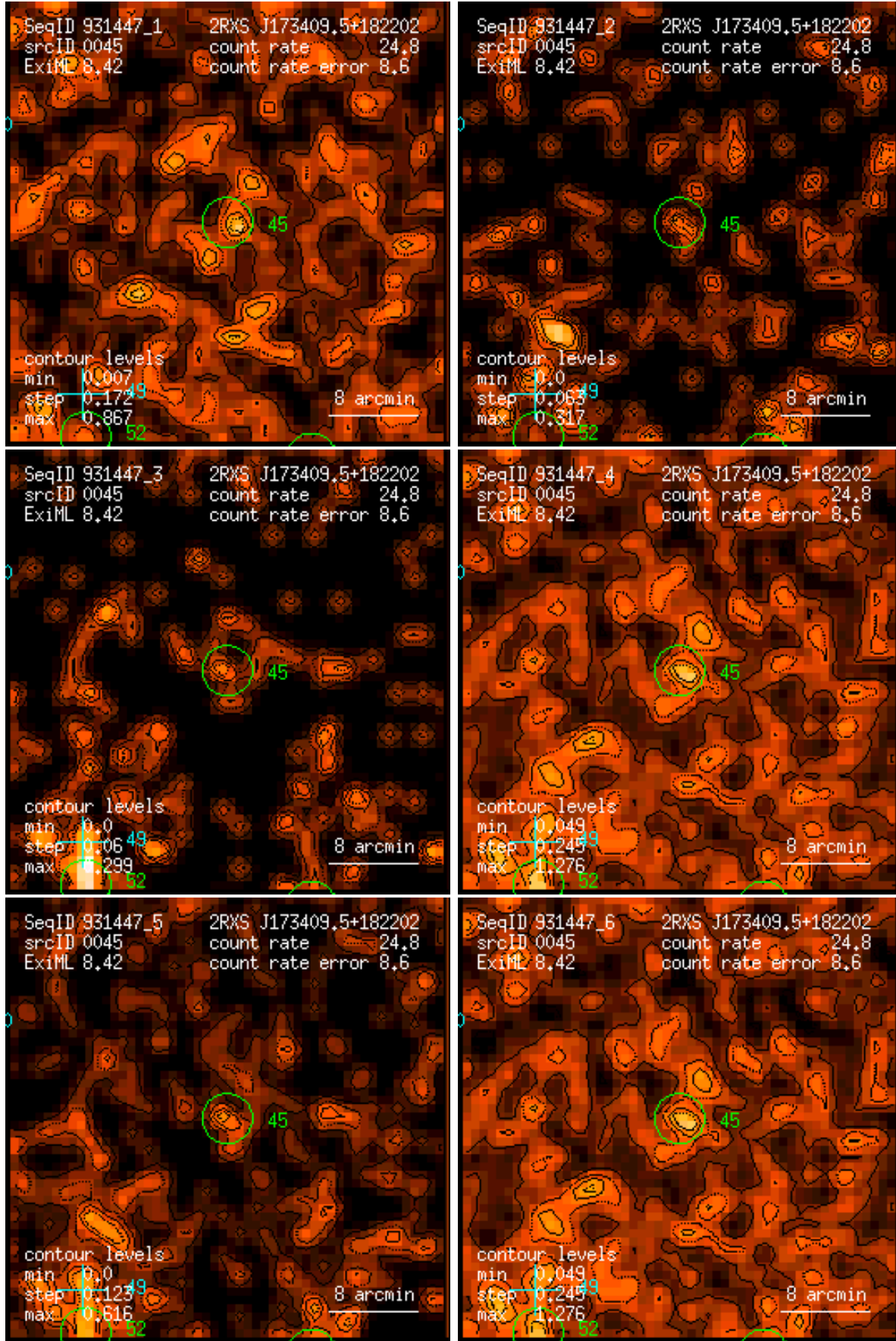
Figure 45: RASS 931447: detection 0045: band rate images, Gaussian filter: (1) PSPC channels 11 – 41, (2) 52 – 90, (3) 91 – 201, (4) 11 – 235, (5) 52 – 201, (6) 11 – 201. Broad band rates in counts/ks. Band rate contour levels in counts/ks/arcmin 2 .
