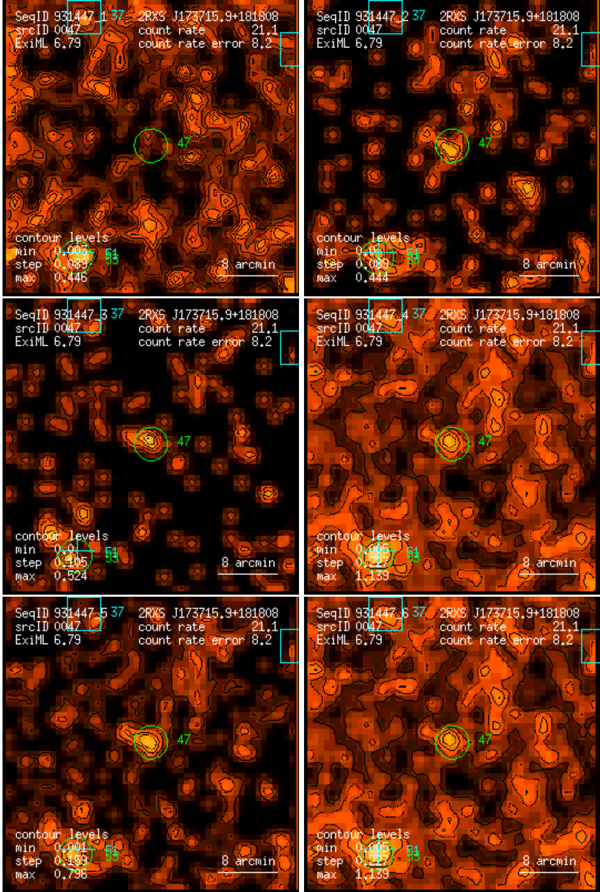
Figure 47: RASS 931447: detection 0047: band rate images, Gaussian filter: (1) PSPC channels 11 – 41, (2) 52 – 90, (3) 91 – 201, (4) 11 – 235, (5) 52 – 201, (6) 11 – 201. Broad band rates in counts/ks. Band rate contour levels in counts/ks/arcmin 2 .
