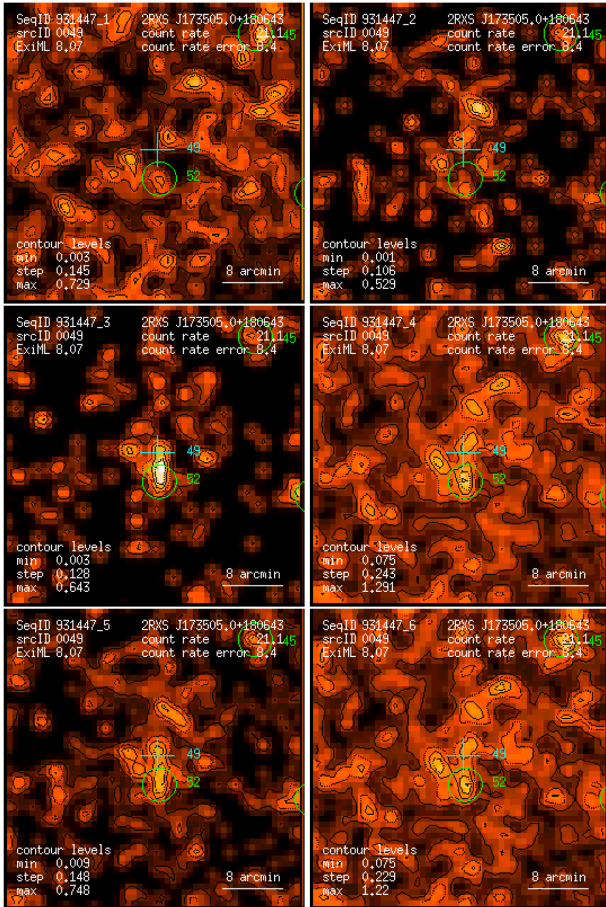
Figure 49: RASS 931447: detection 0049: band rate images, Gaussian filter: (1) PSPC channels 11 – 41, (2) 52 – 90, (3) 91 – 201, (4) 11 – 235, (5) 52 – 201, (6) 11 – 201. Broad band rates in counts/ks. Band rate contour levels in counts/ks/arcmin 2 .
