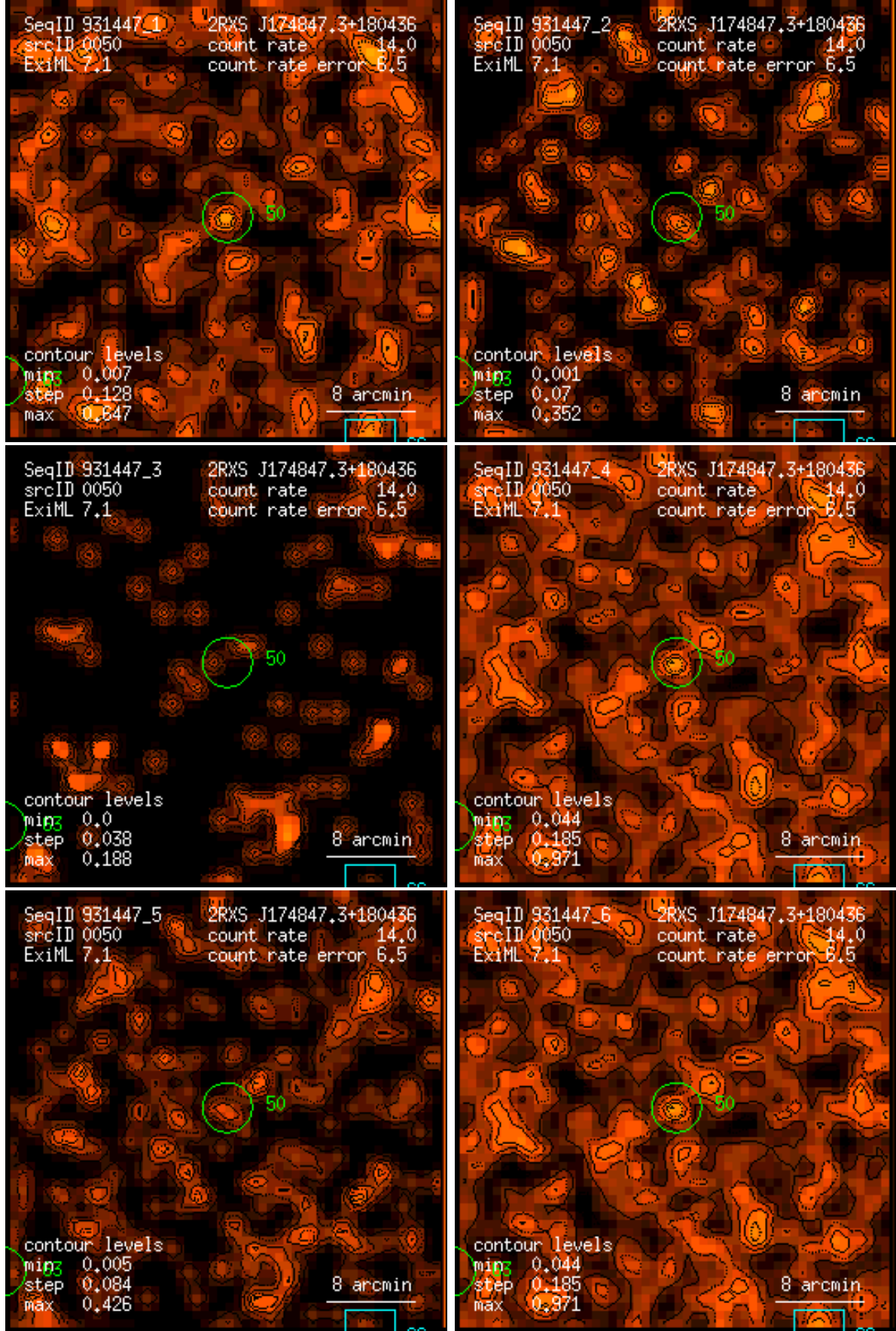
Figure 50: RASS 931447: detection 0050: band rate images, Gaussian filter: (1) PSPC channels 11 – 41, (2) 52 – 90, (3) 91 – 201, (4) 11 – 235, (5) 52 – 201, (6) 11 – 201. Broad band rates in counts/ks. Band rate contour levels in counts/ks/arcmin 2 .
