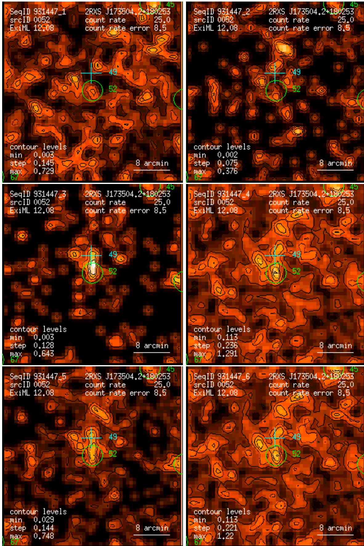
Figure 52: RASS 931447: detection 0052: band rate images, Gaussian filter: (1) PSPC channels 11 – 41, (2) 52 – 90, (3) 91 – 201, (4) 11 – 235, (5) 52 – 201, (6) 11 – 201. Broad band rates in counts/ks. Band rate contour levels in counts/ks/arcmin 2 .
