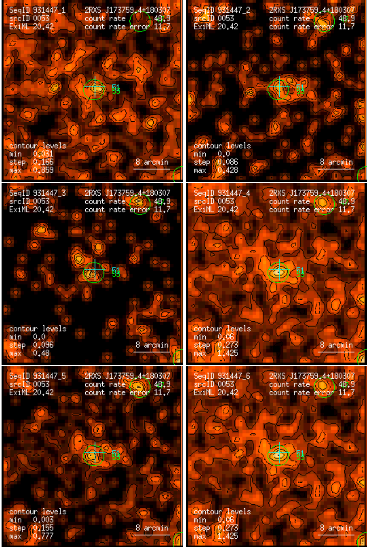
Figure 53: RASS 931447: detection 0053: band rate images, Gaussian filter: (1) PSPC channels 11 – 41, (2) 52 – 90, (3) 91 – 201, (4) 11 – 235, (5) 52 – 201, (6) 11 – 201. Broad band rates in counts/ks. Band rate contour levels in counts/ks/arcmin 2 .
