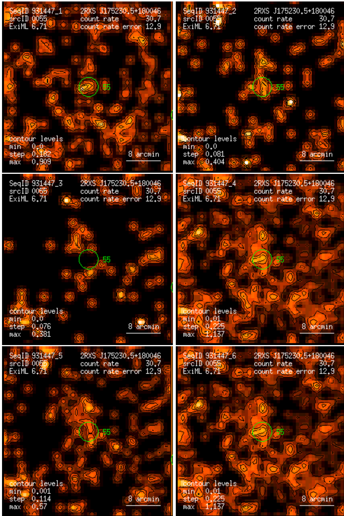
Figure 55: RASS 931447: detection 0055: band rate images, Gaussian filter: (1) PSPC channels 11 – 41, (2) 52 – 90, (3) 91 – 201, (4) 11 – 235, (5) 52 – 201, (6) 11 – 201. Broad band rates in counts/ks. Band rate contour levels in counts/ks/arcmin 2 .
