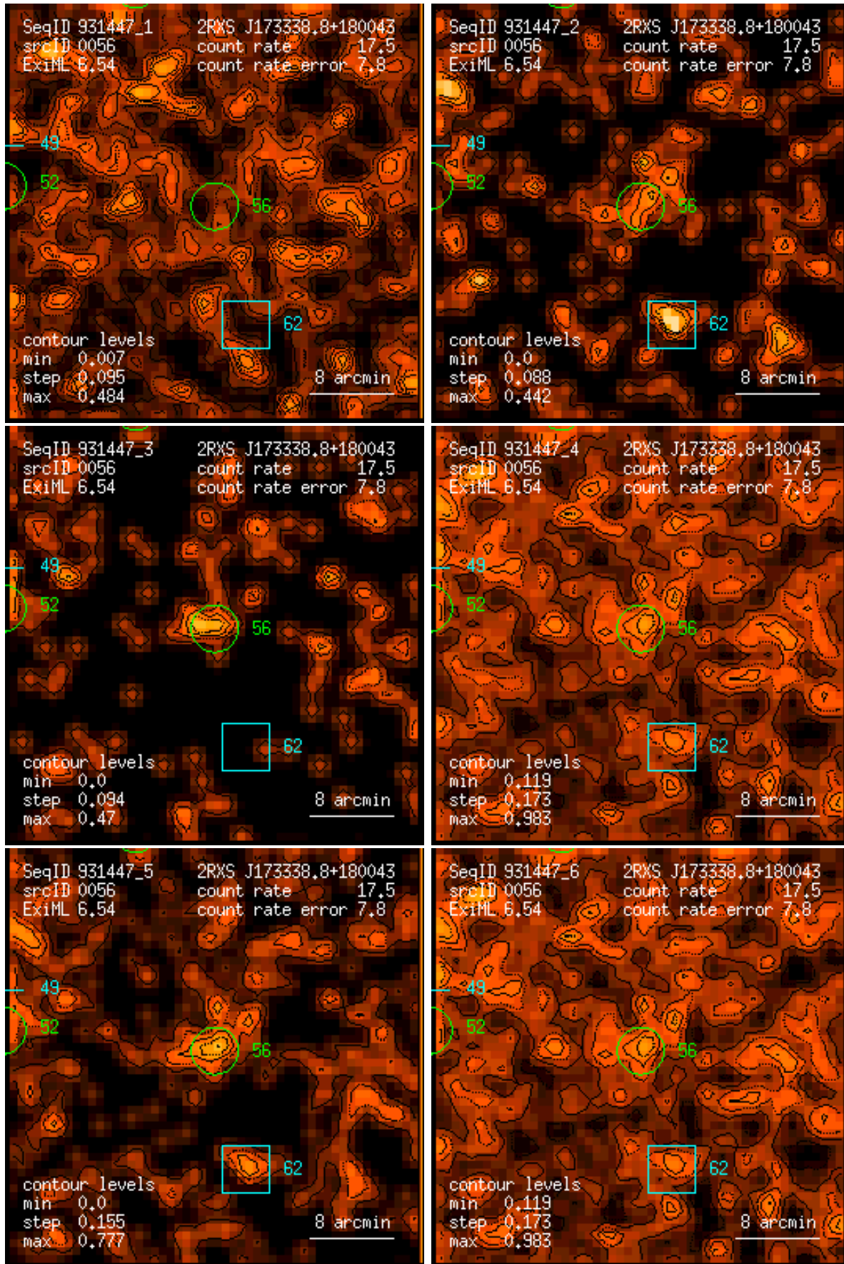
Figure 56: RASS 931447: detection 0056: band rate images, Gaussian filter: (1) PSPC channels 11 – 41, (2) 52 – 90, (3) 91 – 201, (4) 11 – 235, (5) 52 – 201, (6) 11 – 201. Broad band rates in counts/ks. Band rate contour levels in counts/ks/arcmin 2 .
