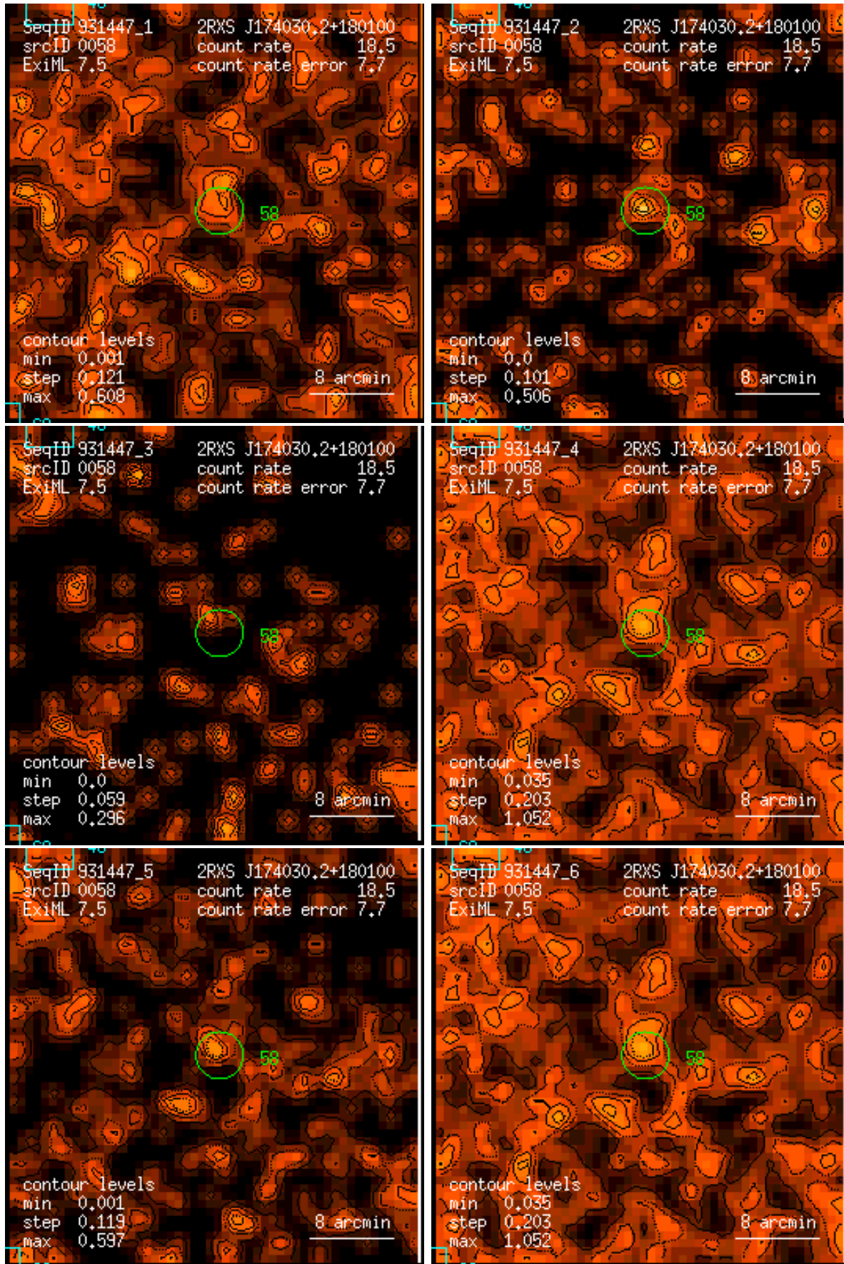
Figure 58: RASS 931447: detection 0058: band rate images, Gaussian filter: (1) PSPC channels 11 – 41, (2) 52 – 90, (3) 91 – 201, (4) 11 – 235, (5) 52 – 201, (6) 11 – 201. Broad band rates in counts/ks. Band rate contour levels in counts/ks/arcmin 2 .
