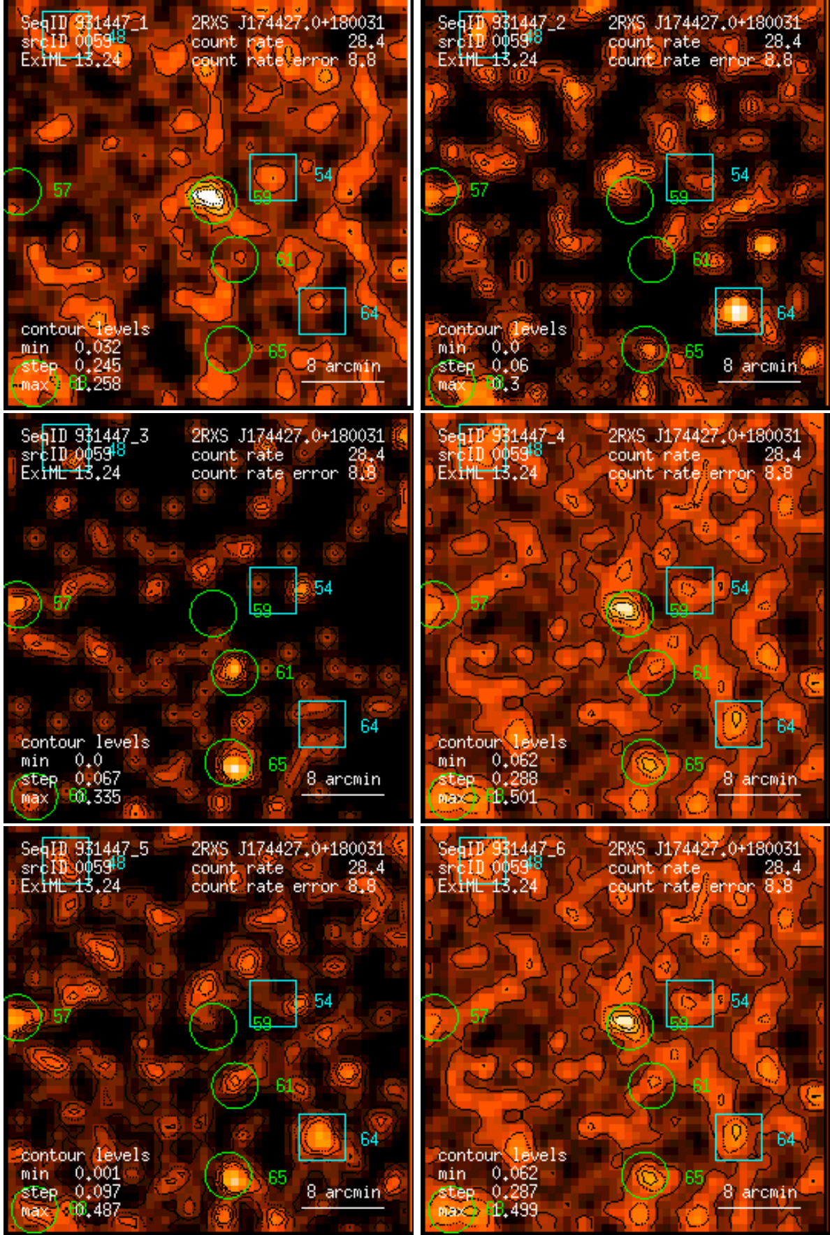
Figure 59: RASS 931447: detection 0059: band rate images, Gaussian filter: (1) PSPC channels 11 – 41, (2) 52 – 90, (3) 91 – 201, (4) 11 – 235, (5) 52 – 201, (6) 11 – 201. Broad band rates in counts/ks. Band rate contour levels in counts/ks/arcmin 2 .
