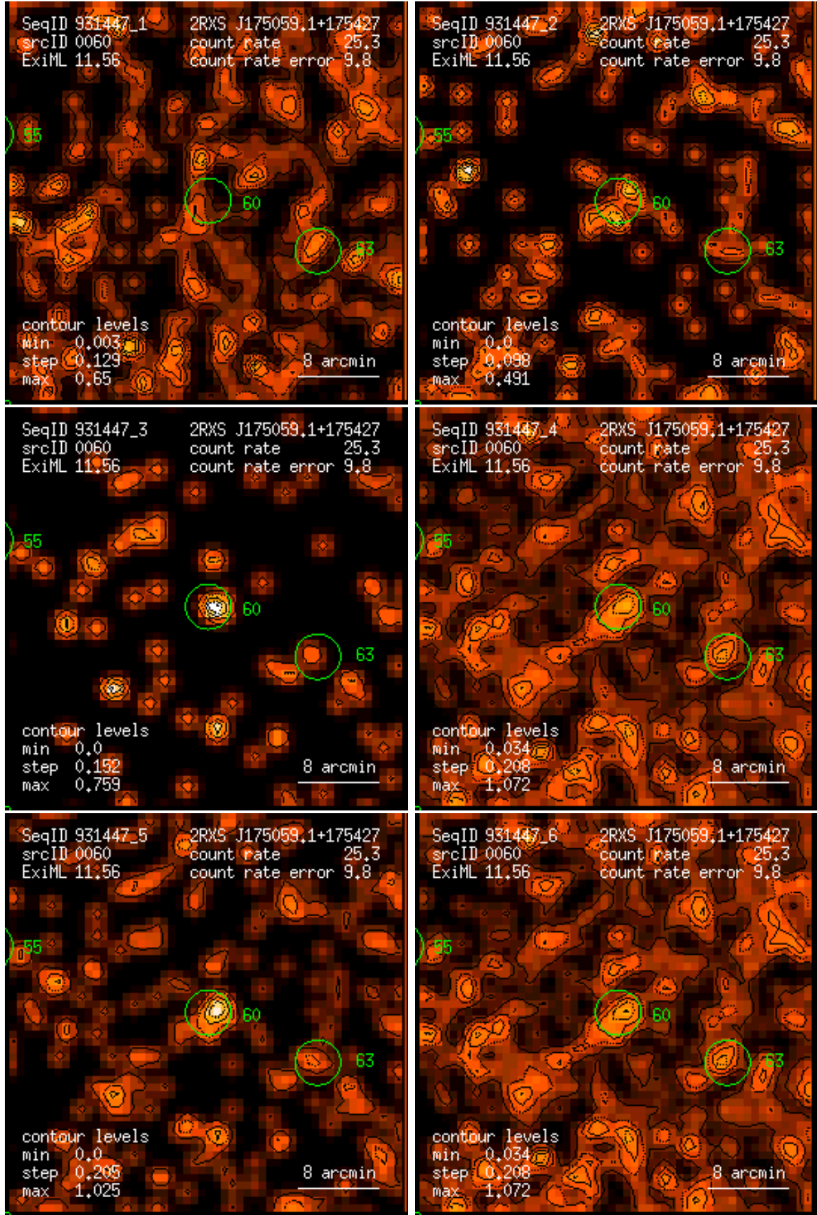
Figure 60: RASS 931447: detection 0060: band rate images, Gaussian filter: (1) PSPC channels 11 – 41, (2) 52 – 90, (3) 91 – 201, (4) 11 – 235, (5) 52 – 201, (6) 11 – 201. Broad band rates in counts/ks. Band rate contour levels in counts/ks/arcmin 2 .
