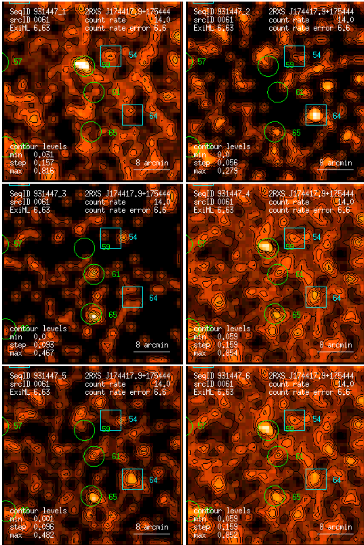
Figure 61: RASS 931447: detection 0061: band rate images, Gaussian filter: (1) PSPC channels 11 – 41, (2) 52 – 90, (3) 91 – 201, (4) 11 – 235, (5) 52 – 201, (6) 11 – 201. Broad band rates in counts/ks. Band rate contour levels in counts/ks/arcmin 2 .
