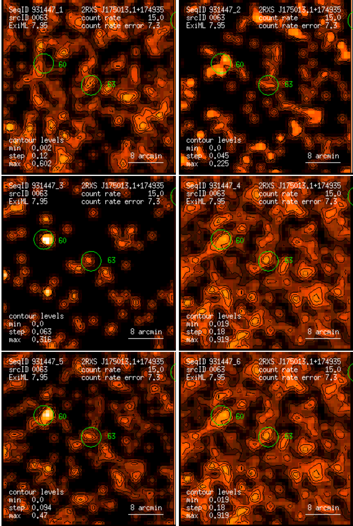
Figure 63: RASS 931447: detection 0063: band rate images, Gaussian filter: (1) PSPC channels 11 – 41, (2) 52 – 90, (3) 91 – 201, (4) 11 – 235, (5) 52 – 201, (6) 11 – 201. Broad band rates in counts/ks. Band rate contour levels in counts/ks/arcmin 2 .
