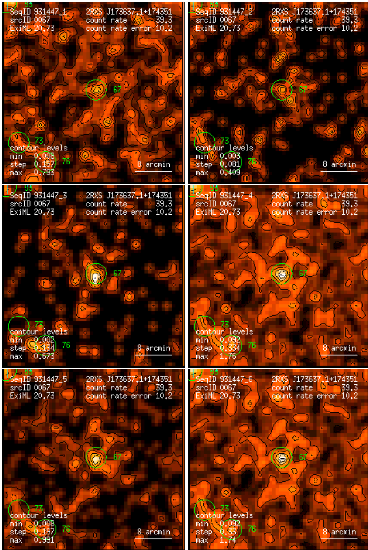
Figure 67: RASS 931447: detection 0067: band rate images, Gaussian filter: (1) PSPC channels 11 – 41, (2) 52 – 90, (3) 91 – 201, (4) 11 – 235, (5) 52 – 201, (6) 11 – 201. Broad band rates in counts/ks. Band rate contour levels in counts/ks/arcmin 2 .
