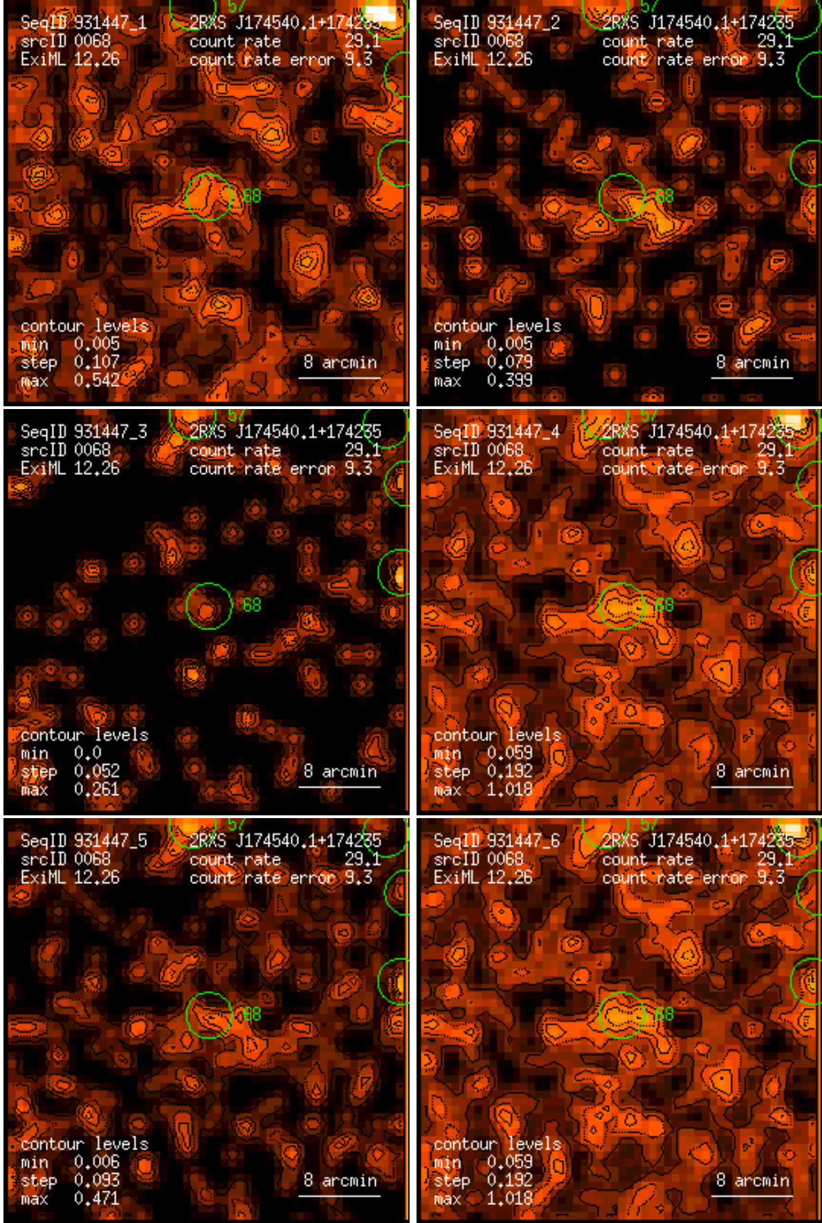
Figure 68: RASS 931447: detection 0068: band rate images, Gaussian filter: (1) PSPC channels 11 – 41, (2) 52 – 90, (3) 91 – 201, (4) 11 – 235, (5) 52 – 201, (6) 11 – 201. Broad band rates in counts/ks. Band rate contour levels in counts/ks/arcmin 2 .
