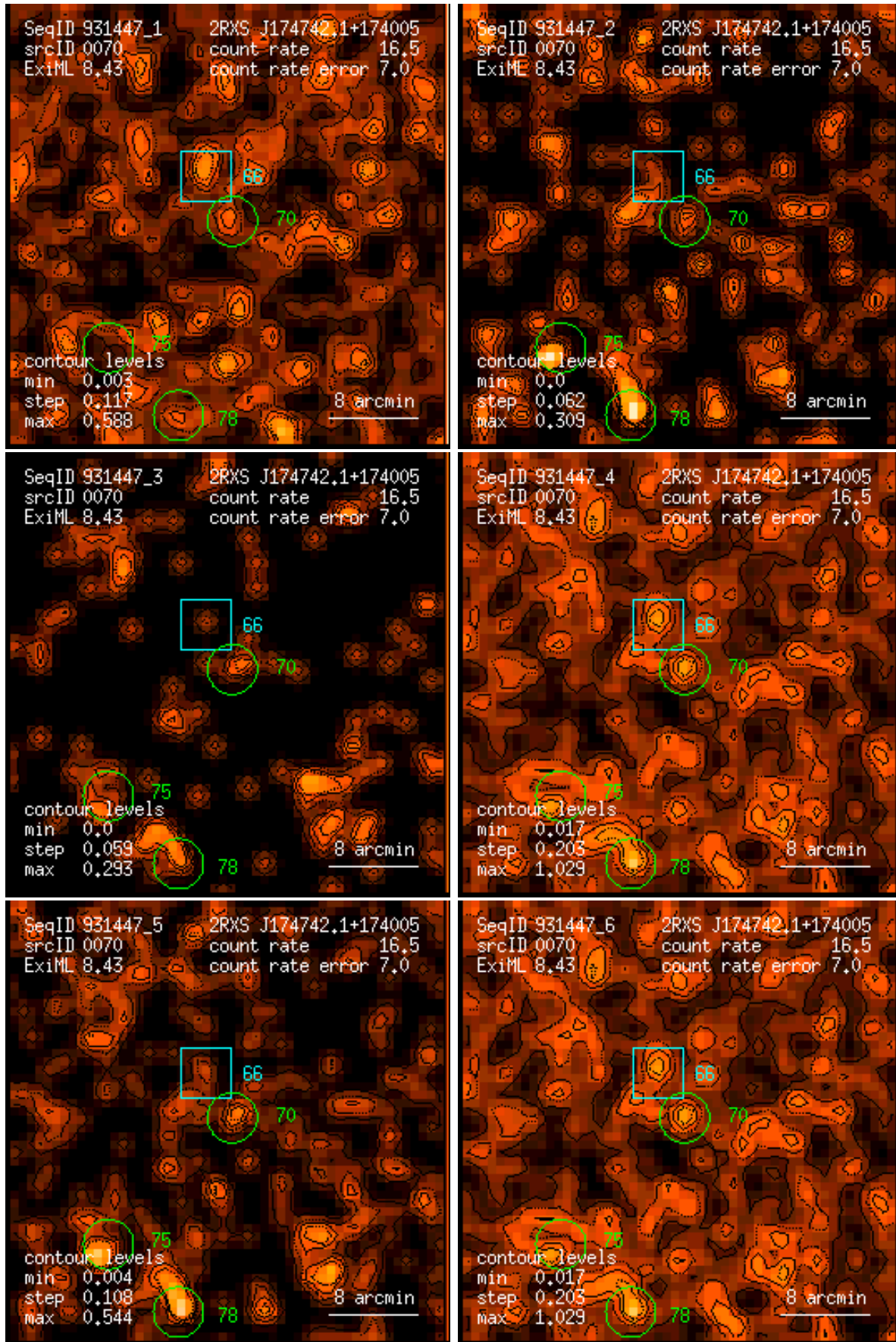
Figure 70: RASS 931447: detection 0070: band rate images, Gaussian filter: (1) PSPC channels 11 – 41, (2) 52 – 90, (3) 91 – 201, (4) 11 – 235, (5) 52 – 201, (6) 11 – 201. Broad band rates in counts/ks. Band rate contour levels in counts/ks/arcmin 2 .
