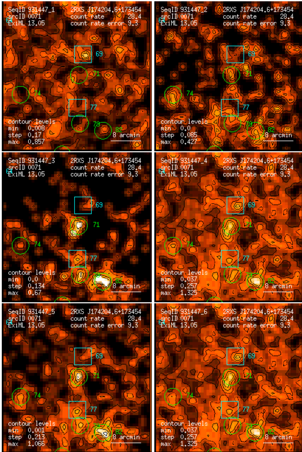
Figure 71: RASS 931447: detection 0071: band rate images, Gaussian filter: (1) PSPC channels 11 – 41, (2) 52 – 90, (3) 91 – 201, (4) 11 – 235, (5) 52 – 201, (6) 11 – 201. Broad band rates in counts/ks. Band rate contour levels in counts/ks/arcmin 2 .
