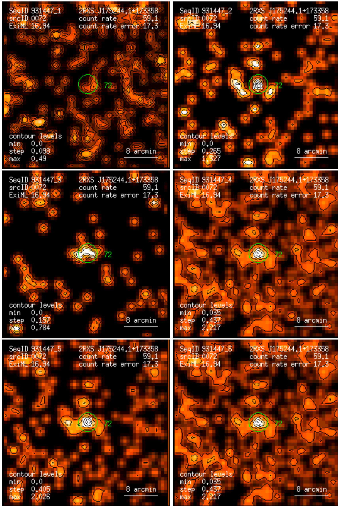
Figure 72: RASS 931447: detection 0072: band rate images, Gaussian filter: (1) PSPC channels 11 – 41, (2) 52 – 90, (3) 91 – 201, (4) 11 – 235, (5) 52 – 201, (6) 11 – 201. Broad band rates in counts/ks. Band rate contour levels in counts/ks/arcmin 2 .
