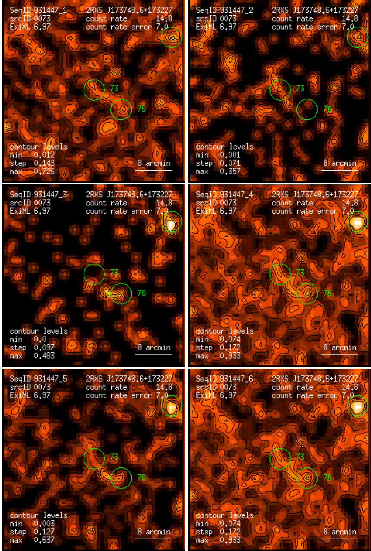
Figure 73: RASS 931447: detection 0073: band rate images, Gaussian filter: (1) PSPC channels 11 – 41, (2) 52 – 90, (3) 91 – 201, (4) 11 – 235, (5) 52 – 201, (6) 11 – 201. Broad band rates in counts/ks. Band rate contour levels in counts/ks/arcmin 2 .
