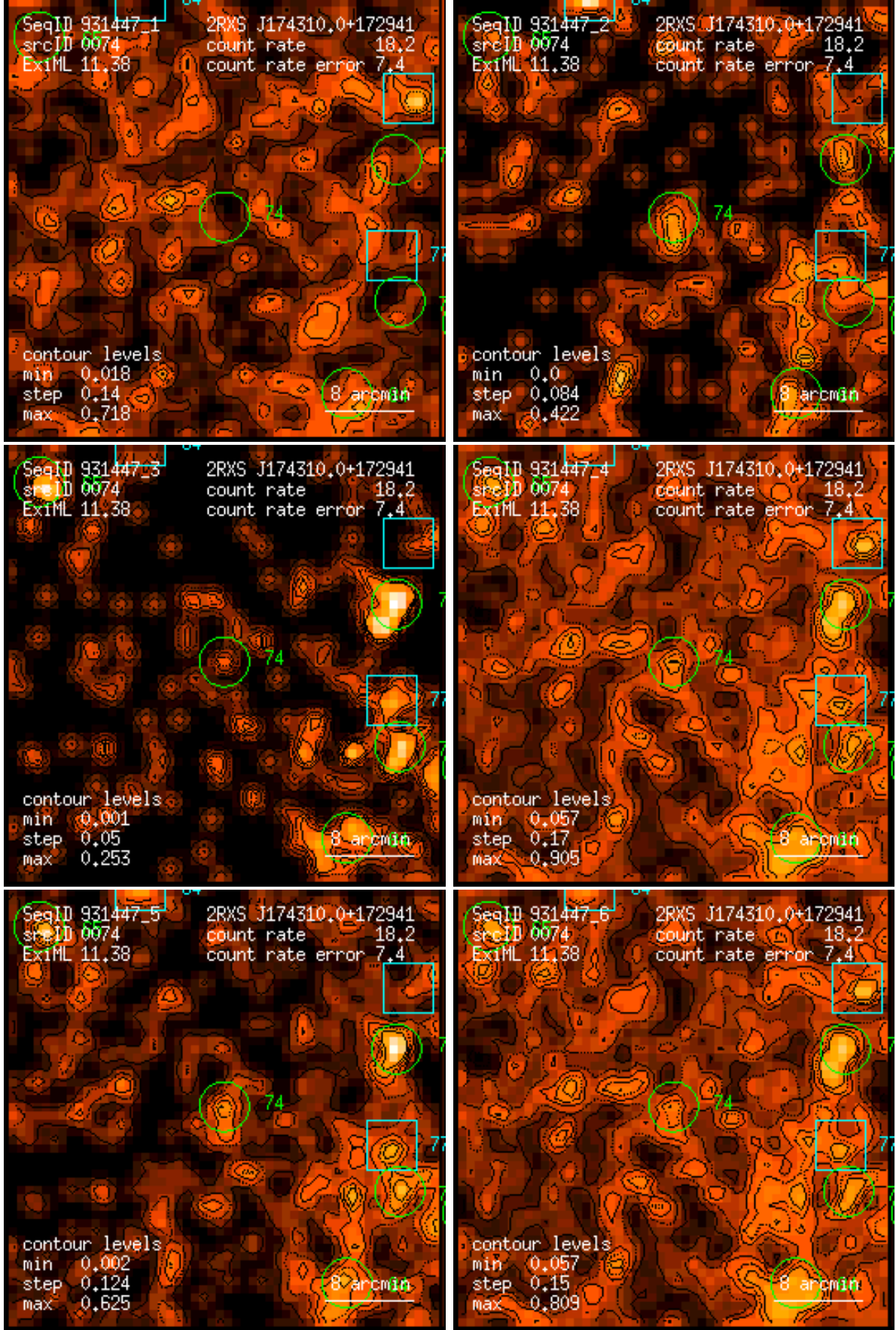
Figure 74: RASS 931447: detection 0074: band rate images, Gaussian filter: (1) PSPC channels 11 – 41, (2) 52 – 90, (3) 91 – 201, (4) 11 – 235, (5) 52 – 201, (6) 11 – 201. Broad band rates in counts/ks. Band rate contour levels in counts/ks/arcmin 2 .
