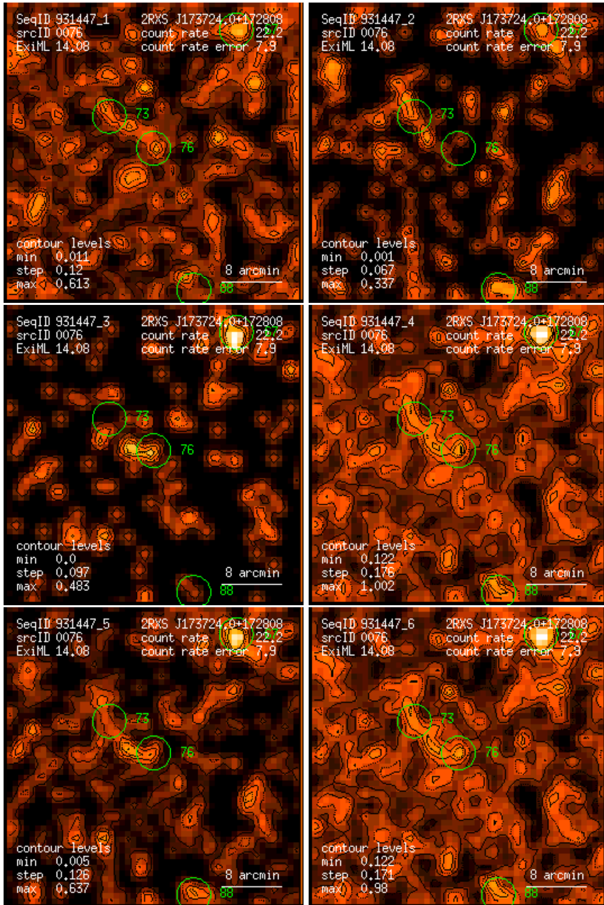
Figure 76: RASS 931447: detection 0076: band rate images, Gaussian filter: (1) PSPC channels 11 – 41, (2) 52 – 90, (3) 91 – 201, (4) 11 – 235, (5) 52 – 201, (6) 11 – 201. Broad band rates in counts/ks. Band rate contour levels in counts/ks/arcmin 2 .
