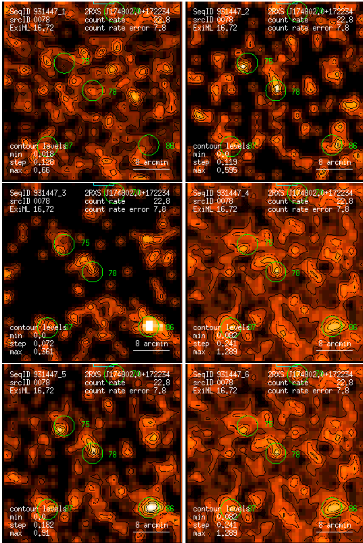
Figure 78: RASS 931447: detection 0078: band rate images, Gaussian filter: (1) PSPC channels 11 – 41, (2) 52 – 90, (3) 91 – 201, (4) 11 – 235, (5) 52 – 201, (6) 11 – 201. Broad band rates in counts/ks. Band rate contour levels in counts/ks/arcmin 2 .
